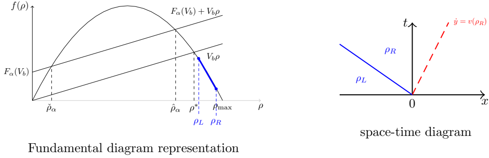
Figure 7: The solution of the constrained Riemann problem of (1) with \rho^* < \rho_L < \rho_R : case iii of Definition 2.
