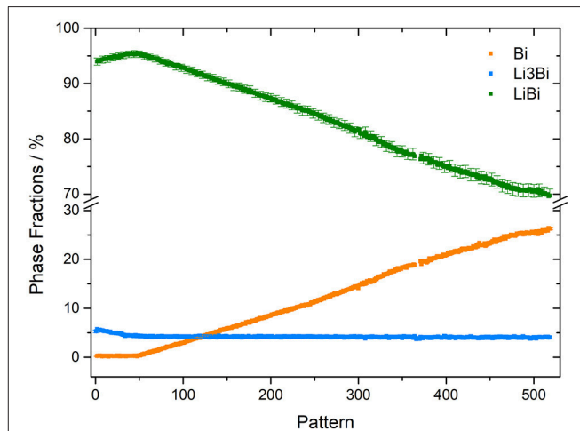
FIGURE 4 | Phase fractions as a function of pattern number as determined by Rietveld refinement.
