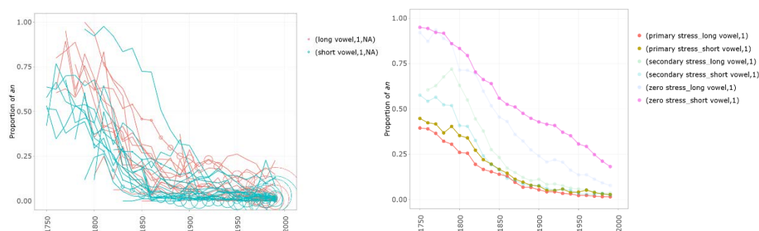
Figure 12: Proportion of an : a for borrowed <h>-initial lemmas without /j/ grouped by initial stress level and vowel quantity. Left panel: Plotting individual items and scaling shape according to frequency. Right panel: Plotting groups and adjusting opacity according to total frequency.
