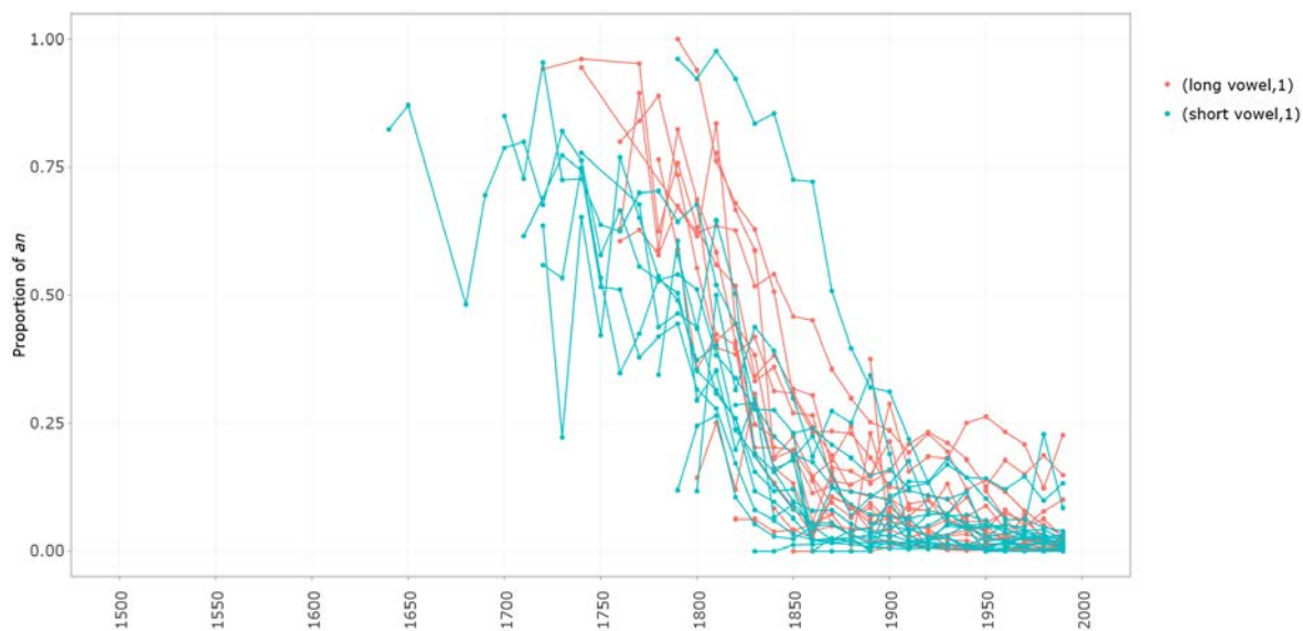
Figure 11: Proportion of an : a for borrowed <h>-initial lemmas without /j/. Plotting individual items, grouped by initial stress level and vowel quantity.
