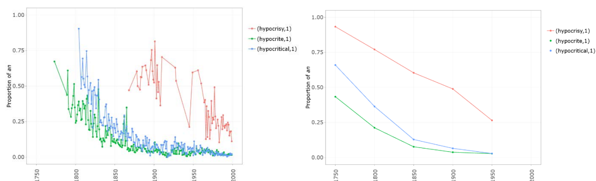
Figure 13: Proportion of an : a for hypocrisy , hypocrite and hypocritical . Left panel: Aggregation baseline set to 1 year. Right panel: Aggregation baseline set to 50 years.
