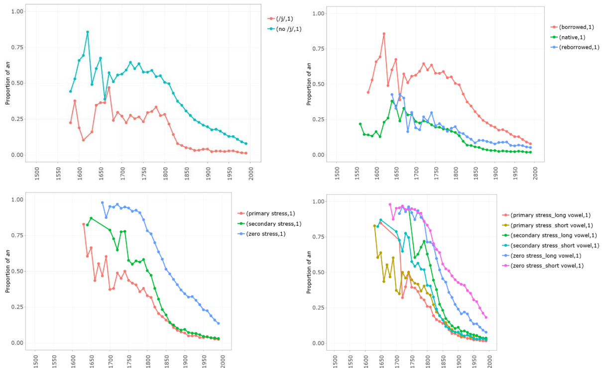
Figure 10: Proportion of an : a for <h>-initial lemmas. Top left panel: Borrowed words, grouped by presence/absence of /j/. Top right panel: Words without /j/, grouped by etymological origin. Bottom left panel: Borrowed words without /j/, grouped by initial syllable stress. Bottom right panel: Borrowed words without /j/, grouped by initial stress level and vowel quantity.
