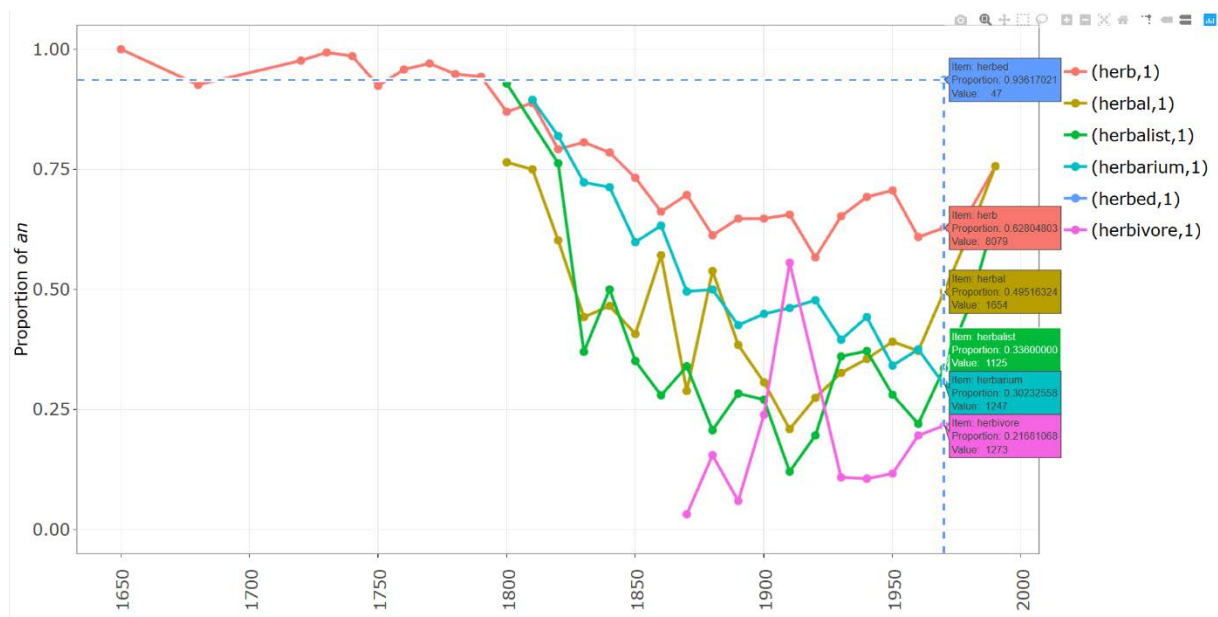
Figure 5: Interactive plot with display options [Toggle spike lines] and [Compare data on hover] activated.
