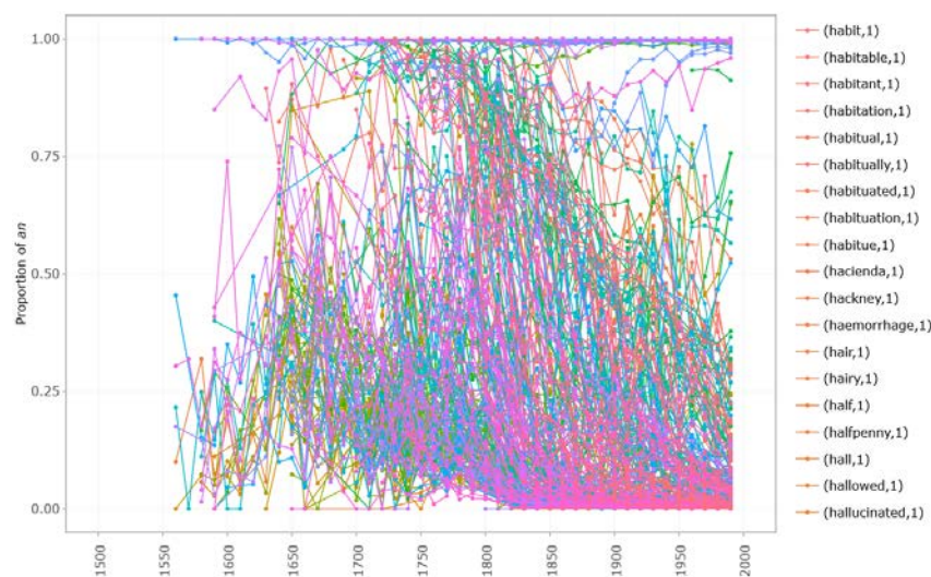
Figure 8: Proportion of an : a for all <h>-initial lemmas, ungrouped.
