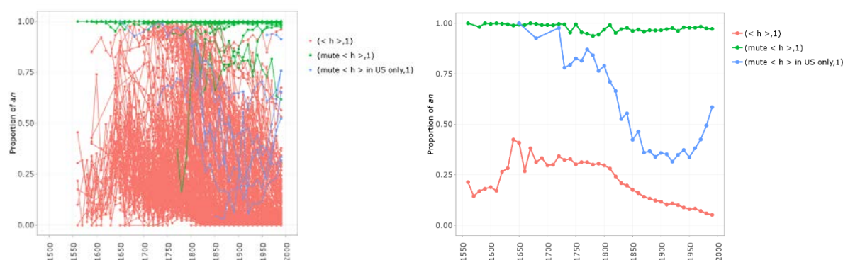
Figure 9: Proportion of an : a for all <h>-initial lemmas, grouped by onset type. Left panel: Plotting individual items. Right panel: Plotting aggregated data per group.
