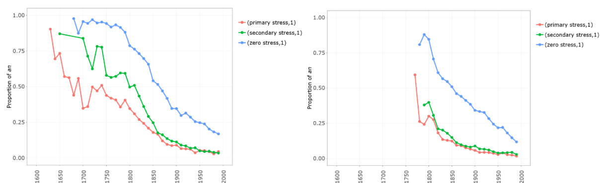
Figure 7: Proportion of an : a for borrowed <h>-initial lemmas without /j/ grouped by initial stress. Left panel: Filter set to GB. Right panel: Filter set to US.
