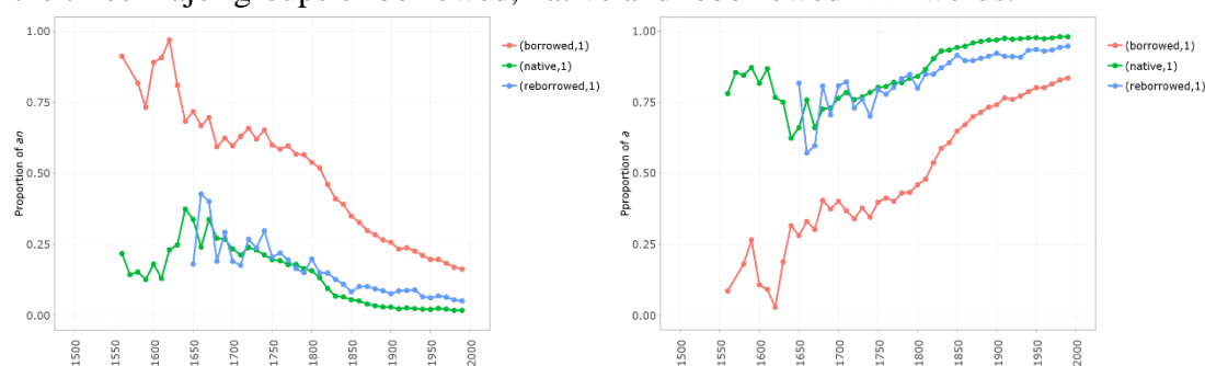
Figure 2: Proportions of article allomorphs for the groups of borrowed, native and reborrowed <h>-initial words. Left panel: Proportion of an : a . Right panel: Proportion of a : an . Click on a figure for a high-resolution version.
