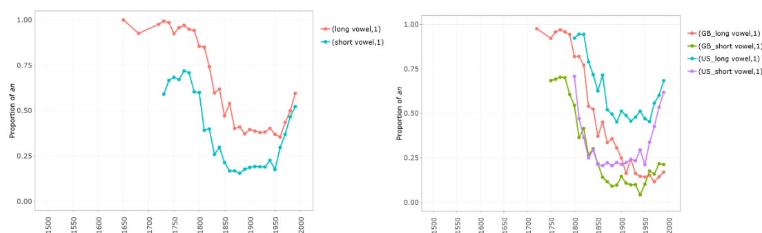
Figure 3: Proportion of an : a for the group herb , herbal , herbalist , herbarium , herbicide , herbivore , herbed (labelled ‘long vowel’) and the item homage (labelled ‘short vowel’). Left panel: All data. Right panel: GB and US separated.
