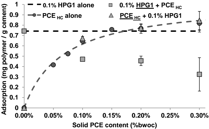
Fig. 6. Adsorption isotherms of HPG1 alone (---), PCE HC alone (—●—), HPG1 (■) and PCE HC (Δ) when they are combined.
