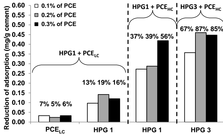
Fig. 8. Reduction in the adsorption of: PCE LC and HPG1 when they are introduced together, and HPG1 and HPG3 when they are combined with PCE HC . The results are expressed in mg/g of cement and in percentage in relation to the adsorption of the admixture introduced alone.
