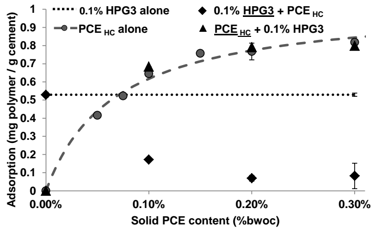
Fig. 7. Adsorption isotherms of HPG3 alone (.....), PCE HC alone (---●---), HPG3 (◆) and PCE HC (▲) when they are combined.
