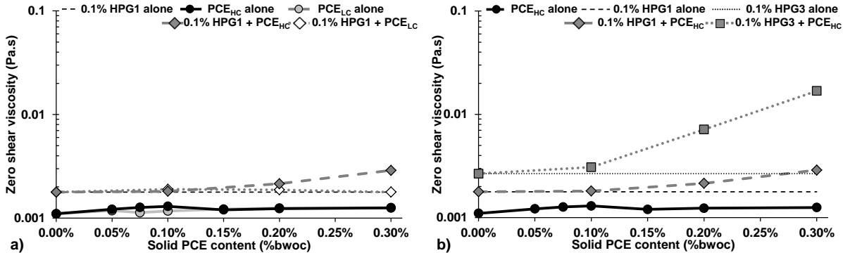
Fig. 11. Evolution of the aqueous phase zero-shear viscosity as a function of the PCE dosage: (a) HPG1 with PCE HC and PCE LC (0.1% HPG1 alone (---), PCE HC alone (—●—), PCE LC alone (—○—), 0.1% HPG1 + PCE HC (—◆—) and 0.1% HPG1 + PCE LC (—◇—)), (b) HPG1 and HPG3 with PCE HC (0.1% HPG1 alone (---), 0.1% HPG3 alone (.....), PCE HC alone (—●—), 0.1% HPG1 + PCE HC (—◆—) and 0.1% HPG3 + PCE HC (—■—))
