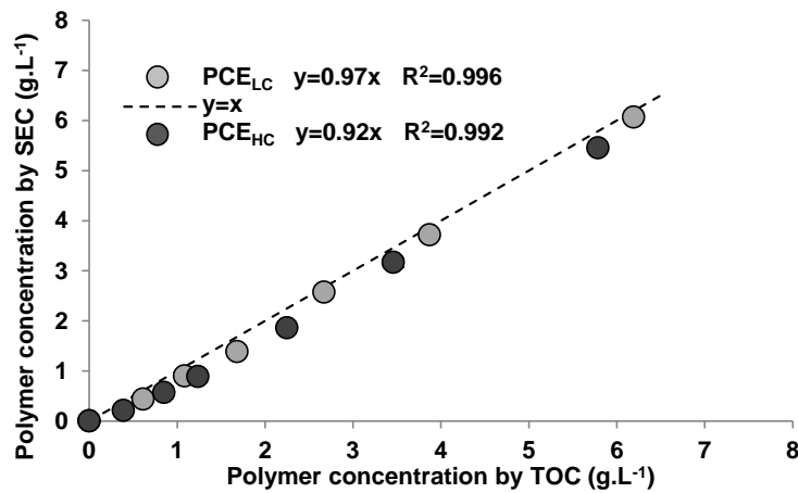
Fig. 3. Validation of the quantification method by correlating the PCE adsorption determined by TOC and SEC methods.
