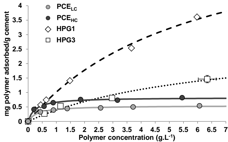
Fig. 4. Adsorption isotherm for PCE LC (○), PCE HC (●), HPG1 (◇) and HPG3 (□).
