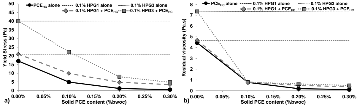
Fig. 10. Effect of the MS HP of the HPG on the yield stress (a) and the residual viscosity (b) when the HPGs (0.1% of HPG1 and 0.1% of HPG3) are combined with PCE HC .
