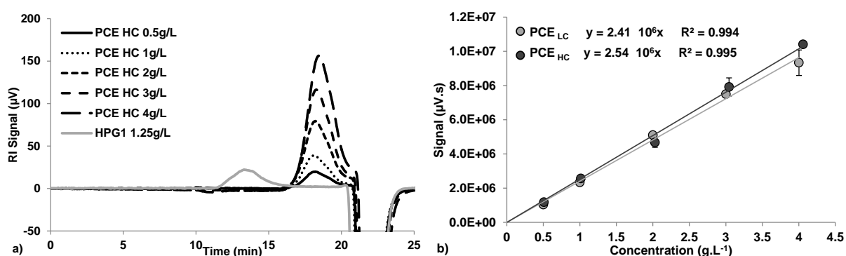
Fig. 2. Illustration of SEC analysis for different concentrations in PCE HC (0.5 to 4 g/L) and for HPG1 (1.25g/L) (a), calibration curves obtained from chromatograms for PCE LC and PCE HC (b).
