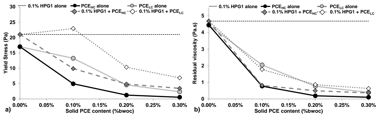
Fig. 9. Effect of the PCE charge density (PCE LC and PCE HC ) on the yield stress (a) and the residual viscosity (b), with or without 0.1% of HPG1.
