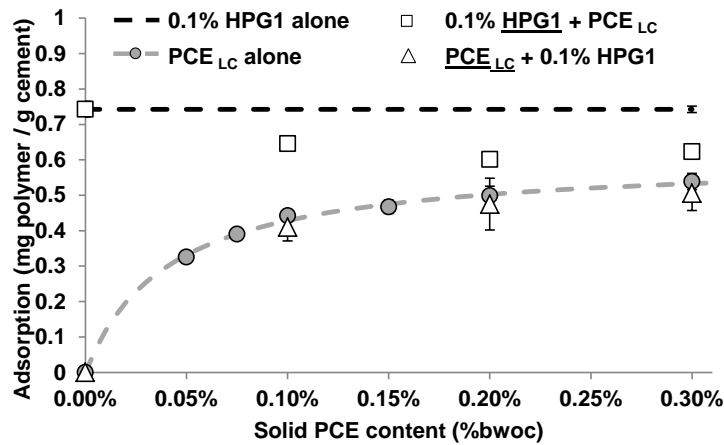
Fig. 5. Adsorption isotherms of HPG1 alone (---), PCE LC alone (—○—), HPG1 (□) and PCE LC (Δ) when they are combined.
