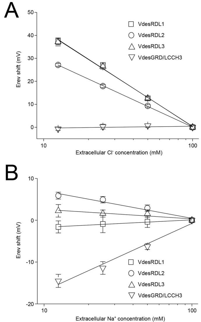
Figure 3. Semi-logarithmic plots showing the effects of the variation of extracellular chloride (A) or sodium (B) concentration on the reversal potential of the current evoked by GABA (EC 30-50 ) determined in X. laevis oocytes that express VdesRDL1, VdesRDL2, VdesRDL3, or VdesGRD/LCCH3. The data are the means \pm S.E. of n = 4–7 oocytes.
