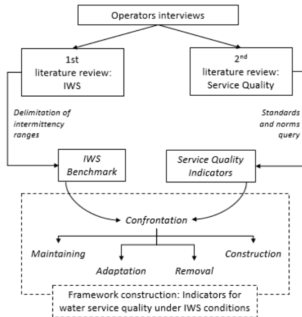
Figure 1. Approach Framework.
