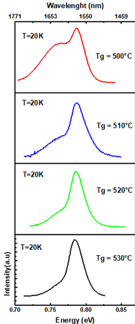
Fig. 10. LTPL spectra collected at 20 K on 350 nm thick hybrid GaInAs epilayers grown at different growth temperatures.
