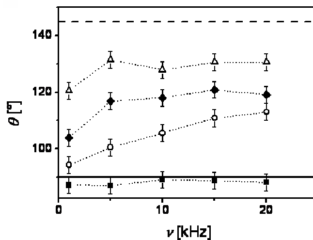
Figure 9. Contact angle \theta versus frequency (see Figure 8 for experimental details). Conductivity: 1850 \mu\text{S}/\text{cm} (squares), 197 \mu\text{S}/\text{cm} (circles), 91 \mu\text{S}/\text{cm} (diamonds), and 42 \mu\text{S}/\text{cm} (triangles). \theta_Y and \theta are shown as dashed and solid lines, respectively. Reprinted from ref. [57].
