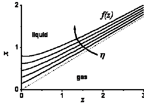
Figure 6. Equilibrium surface profiles. ( \theta=60^\circ ; \eta= 0.2, 0.4, \dots, 1.0 ; \varepsilon_d= 1 ) Reprinted with permission from ref. [49]: Buehrle J., Herminghaus S. and Mugele F., Phys. Rev. Lett. 91, 086101, 2003. Copyright 2003 by the American Physical Society .
