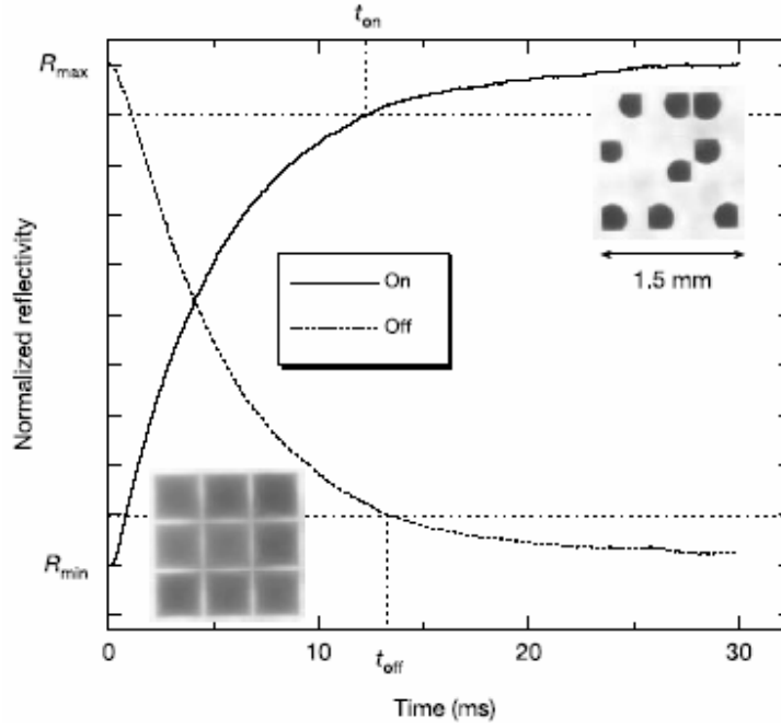
Figure 30. Electrowetting pixel kinetics. Temporal behaviour of a 250 \times 250 \text{ mm}^2 pixel, demonstrating the video-speed response. The oil film thickness is 15 \text{ mm} and the insulator thickness is 0.8 \text{ mm} . The on and off response times are 12 and 13 \text{ ms} respectively. The reflectivity is shown in normalized units, which does not affect the time axis. t_{\text{on}} and t_{\text{off}} are defined as the time it takes to complete 90\% of the optical modulation. Insets, photographs showing the corresponding optical state for a 3 \times 3 array of 500 \times 500 \text{ mm}^2 pixels. (reproduced from ref. [66]).
