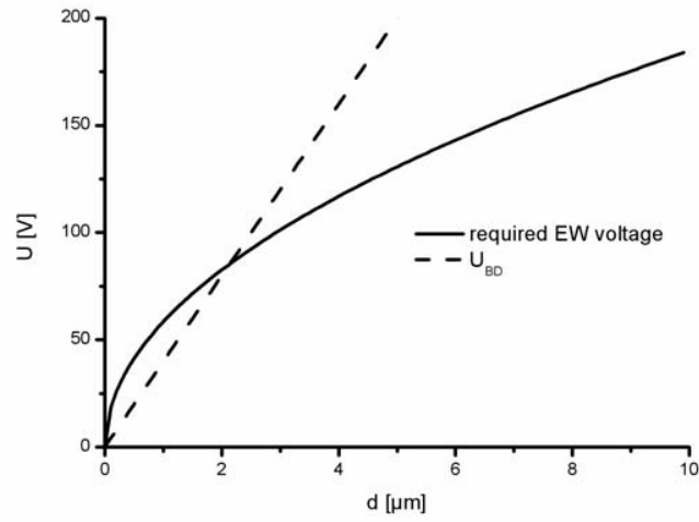
Figure 11. Electrowetting and dielectric breakdown voltage vs. insulator thickness. Solid line: voltage required for a contact angle decrease from 120^\circ (0V) to 70^\circ (for \epsilon_d=2 ; \sigma_{lv}=0.072 \text{ J/m}^2 ). Dashed line: Critical voltage for dielectric breakdown (for EBD=40 \text{ V}/\mu\text{m} )
