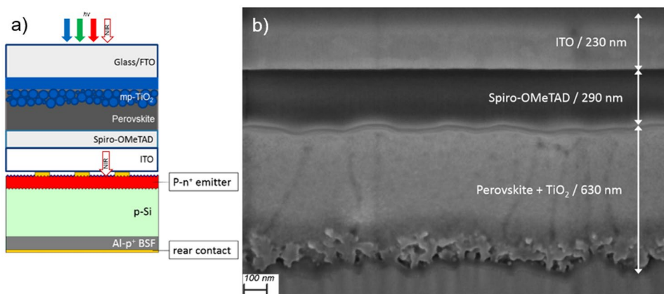
Figure 2. (a) Scheme of the 4-terminal tandem device proposed in this work, with a semitransparent PSC \text{MoO}_x -free with ITO rear contact as top cell and Al-BSF Si solar cell as bottom one to absorb the near infrared (NIR) part of the spectra. (b) Cross-sectional Scanning Electron Microscopy image of a complete semitransparent PSC \text{MoO}_x -free terminated with a 230 nm thick ITO contact, made by Focused Ion Beam polishing and Scanning Electron Microscopy imaging.
