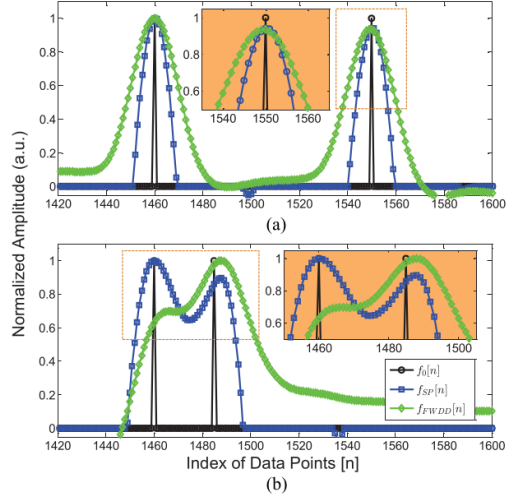
Fig. 1. Comparisons between the assumed (a) f_0[n] and (b) f'_0[n] , and the deconvolution results obtained by sparse deconvolution and FWDD, respectively. Insets are the zoom-in images of corresponding boxed peaks.
