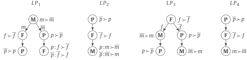
Fig. 1. Four LP-trees.
