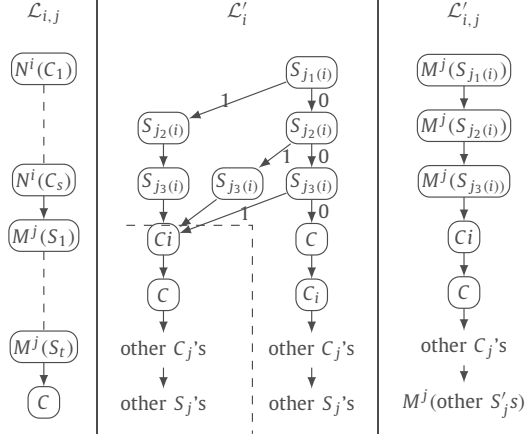
Fig. 7. Reduction of RESTRICTED X3C to K-EVALUATION for Borda with fixed preferences.
