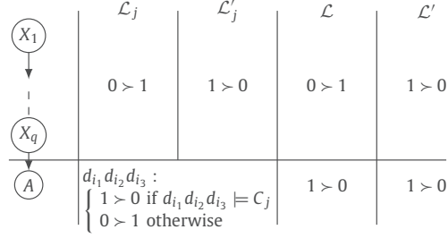
Fig. 5. Reduction of 3SAT to EVALUATION with Borda score and common, unconditional importance.
