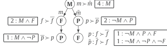
Fig. 3. LP tree LP_1 and its translation into weighted formulas.
