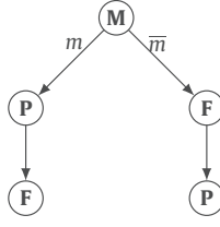
Fig. 6. The importance tree T_1 for Example 7.
