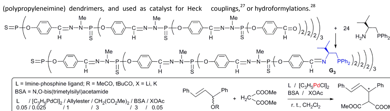
Scheme 3. A 3 rd generation dendrimer bearing P,N ligands, and use of its Pd complex in catalysed asymmetric allylic alkylations.
