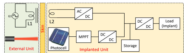
Fig. 1. Schematic of the studied transcutaneous energy transfer systems
