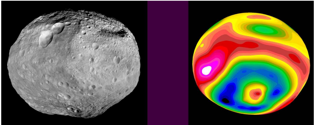
Fig.6. Left: Composite grayscale image of Vesta taken by Dawn spacecraft. Large triple Snowman crater is clearly seen in northern hemisphere. Right: Elevation diagram viewed from the south-east, showing Rheasilvia basin at the Southern pole and Feralia Planitia near the equator (Hubble Space Telescope images). https://en.wikipedia.org/wiki/4_Vesta#/media/File:Vesta_full_mosaic.jpg https://en.wikipedia.org/wiki/File:Vesta-Elevation.jpg
