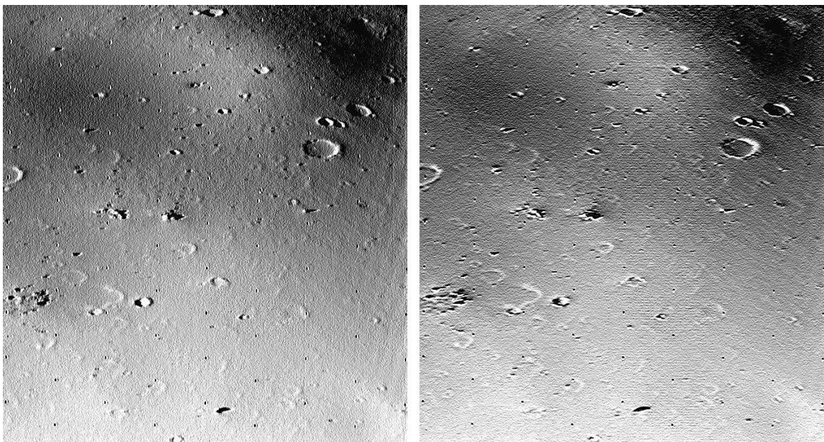
Fig.28. East (left) and South (right) shadowing applied by us to fig.27 reveal surface relief symmetries connected to local stress geometry of upper crustal layers of Deimos..
