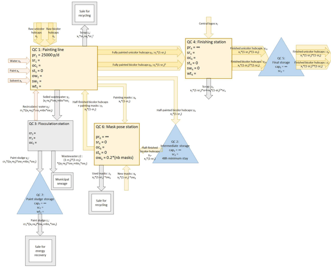
Figure 4 – Painting and finishing subsystem flow inventory
