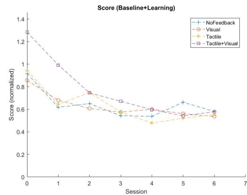
Figure 4: Score on the average of the baseline and learning tries
