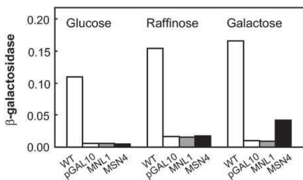
FIG. 2. Ability of CaMSN4 and MNL1 to complement an S. cerevisiae msn2 msn4 double mutation. CaMSN4 and MNL1 were expressed using the ScGAL1 promoter in S. cerevisiae strain Wmsn2msn4 containing a STRE-lacZ reporter. Cells were grown to mid-exponential phase on glucose, raffinose, or galactose and then exposed to 0.3 M NaCl for 30 min, and \beta -galactosidase activities were measured (Miller units). S. cerevisiae W303-1A (WT); S. cerevisiae Wmsn2msn4 containing the empty expression vector pGAL10 (pGAL10); pGAL10-MNL1 (MNL1), or; pGAL10-MSN4 (MSN4). Errors were <10%, and similar data were obtained in three independent experiments.
