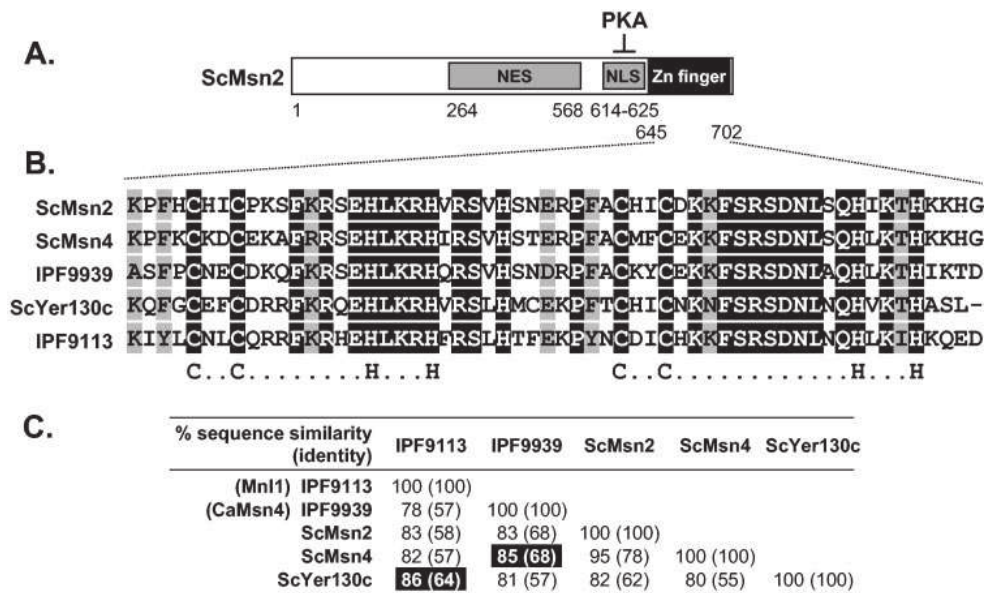
FIG. 1. Comparison of Msn2- and Msn4-like sequences in C. albicans and S. cerevisiae . (A) Cartoon of S. cerevisiae Msn2 (ScMsn2) illustrating the coordinates of the (C_2H_2)_2 DNA binding domain (Zn finger), the nuclear export signal (NES), the NLS, and the repression of the NLS by protein kinase A (PKA) (24). (B) Sequence alignments for the (C_2H_2)_2 regions of the Msn2- and Msn4-like proteins in C. albicans and S. cerevisiae . Residues conserved in all proteins, black; conservative substitutions, grey. (C) Percentage sequence similarities (identities) in these regions. IPF9113 and IPF9939 are most similar to the S. cerevisiae proteins ScYer130c and ScMsn4, respectively.
