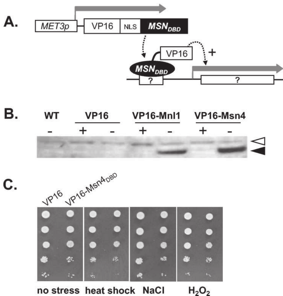
FIG. 9. Expression of a VP16- CaMsn4_{DBD} fusion in C. albicans causes no obvious stress phenotype. (A) Cartoon illustrating the experimental rationale to identify gene targets of CaMsn4 . The CaMET3 promoter is repressed by methionine and cysteine (7). (B) Western blot with anti-VP16 antibody showing regulated expression of MET3-VP16-MSN4 DBD in C. albicans . Wild type, CAI4 (WT; Table 1); SNC11 (VP16); SNC12 (VP16-Mnl1); SNC13 (VP16-Msn4); no methionine or cysteine (-); 10 mM methionine and 10 mM cysteine (+); open arrow, nonspecific band; closed arrow, VP16 fusion protein. (C) Phenotype of C. albicans CAI4 cells expressing VP16- CaMsn4_{DBD} or the VP16 control on plates lacking methionine and cysteine. No stress (SC; 30°C), mild heat shock (25 to 37°C), 1.0 M NaCl, and 2.5 mM H_2O_2 .
