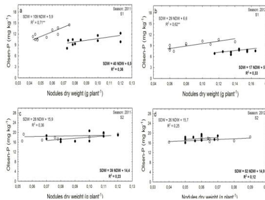
Fig.2. Relationship between nodule biomass and rhizospheresoil Olsen-P of common bean either in intercropping (opened circle) or sole crop (filled circle) under S1 and S2 conditions. asterisks; *, **, *** denote significant difference at p < 0.05 , p < 0.01 and p < 0.001 .
