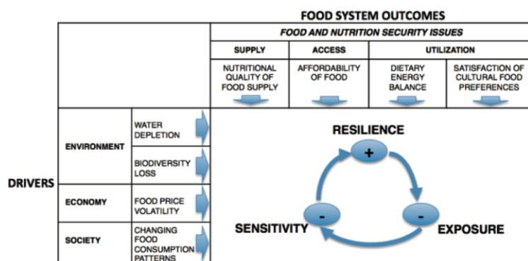
Figure 1: Interactions Drivers of change / Food and Nutrition Security Issues in the Latin Arc (Adapted from: Prospero et al., 2014; Allen & Prospero, 2016)
