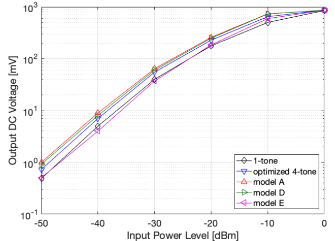
Fig. 3. DC voltage (mV) as a function of the input power (dBm) for specific channel models (A, D, E) of HyperLAN/2 standard.
