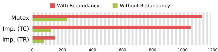
Figure 19: Comparison of the means of reduced and not reduced extracted implications and mutex
