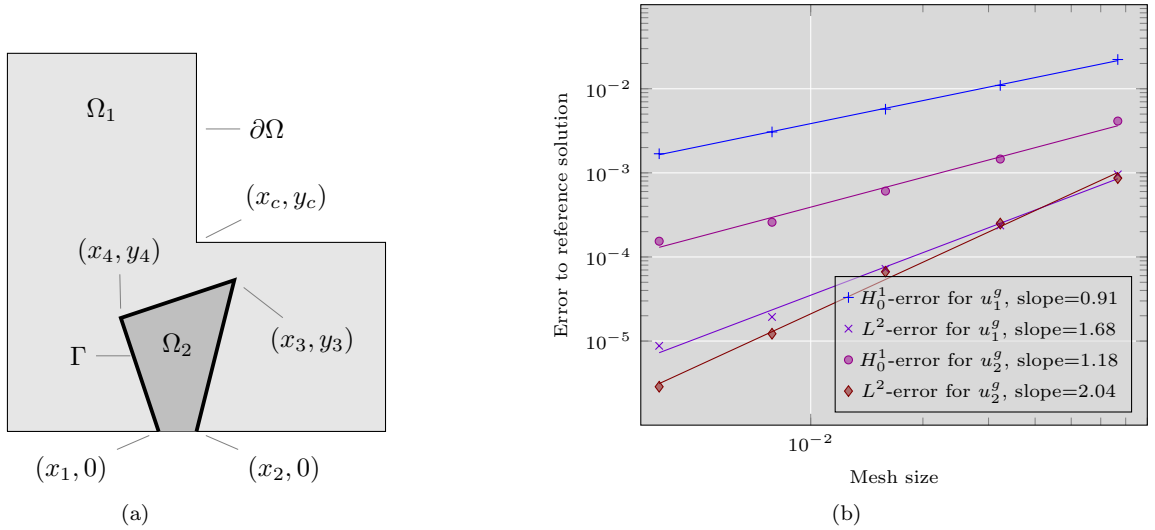
Figure 6: Two dimensional representation of the geometry for the Laplace transmission problem (1) in a L-shape domain (a) and rates of convergence in space for the smooth extension method applied to the resolution of the Laplace transmission problem (1) in a L-shape domain (b).
