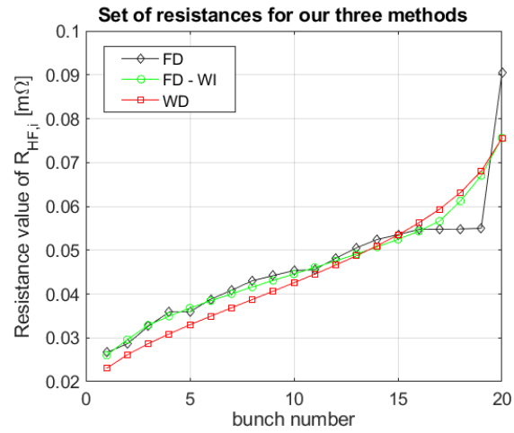
Fig. 5: Difference in resistance values without and with a Weibull initialization for the free set of resistances and for the Weibull set at 1C and 25°C
