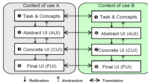
Fig. 1. The Cameleon Reference Framework (from [7])
