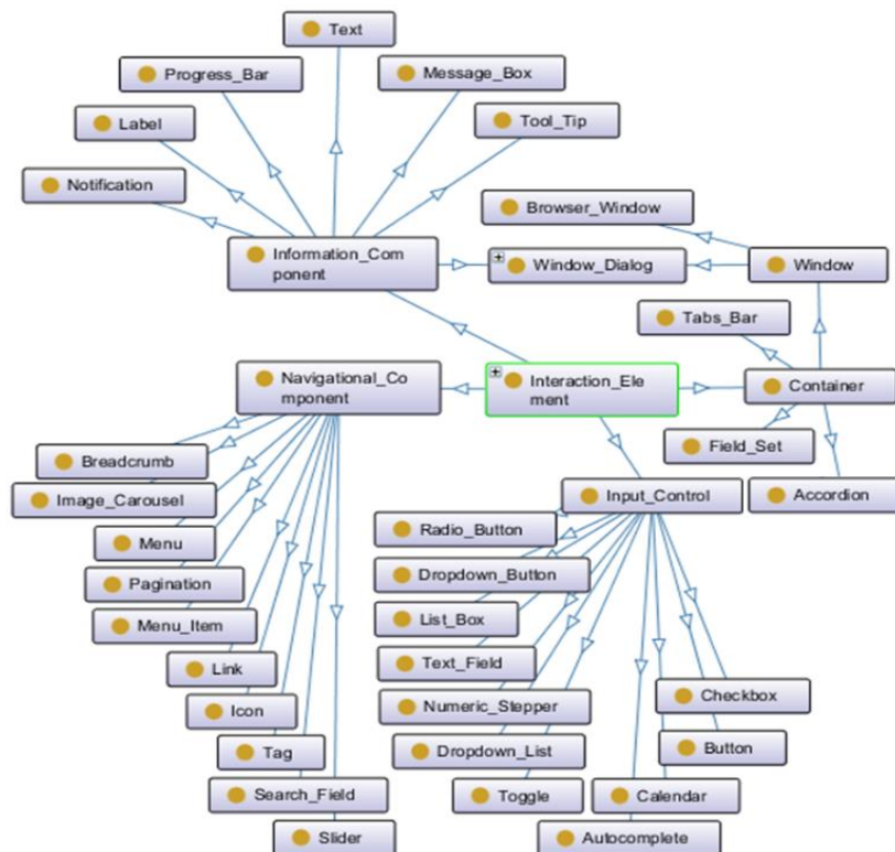
Fig. 6. Graph describing the hierarchy of User Interface (UI) Elements
