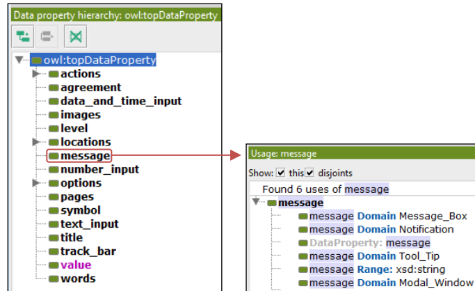
Fig. 5. (a) Left: Data Properties. (b) Right: Data Property “message”
