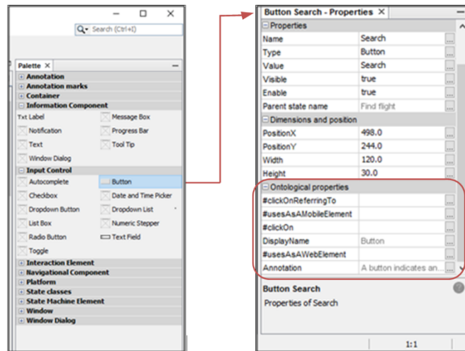
Fig. 12. Palettes with the widget Button and its properties extracted from the ontology
