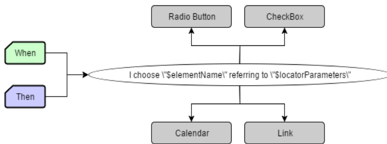
Fig. 10. Components on the ontology used to specify a behavior
