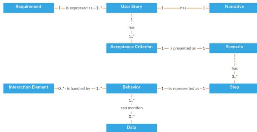
Fig. 2. Conceptual Model of User Requirements
