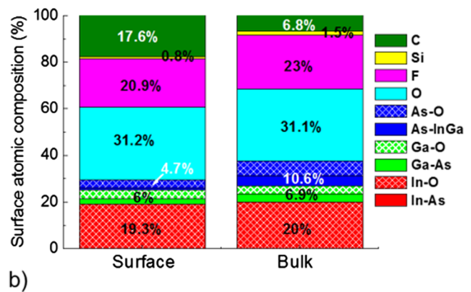
FIG. 3. Atomic composition of the InGaAs surface at grazing angle 76.75^\circ (surface) and near normal angle 23.25^\circ (bulk) before and (b) after He implantation. The percentage indicated on the graph represents the relative chemical quantification of one element whatever its chemical environment.
