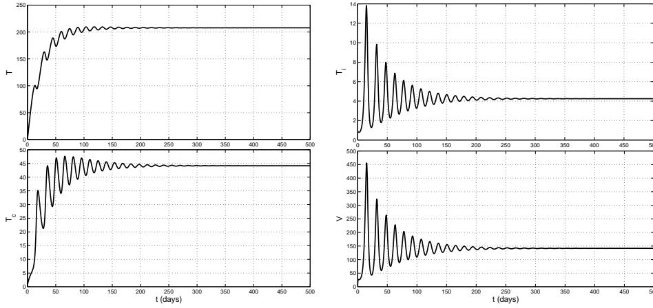
Figure 2 – The time series of model (1) for \tau_i = 0, i = 1, 2, 3, 4 . The chronic infection equilibrium E^* is asymptotically stable when.
