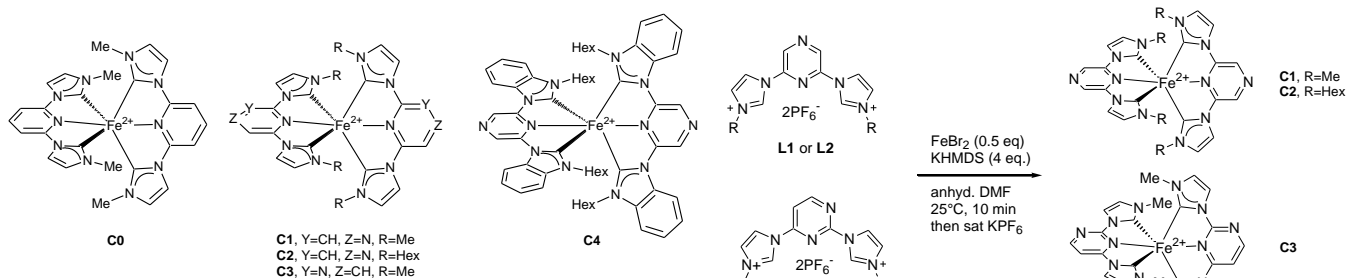
Fig. 1 Complexes studied in this work. In all cases, counter ion is \text{PF}_6^- in any case
