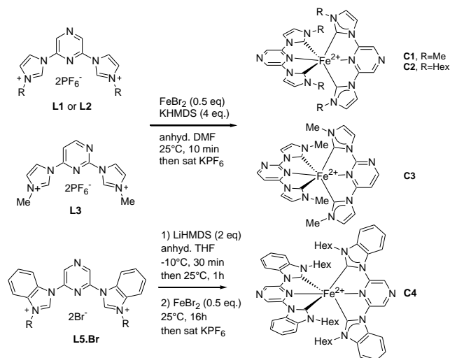
Scheme 2. Synthesis of Complexes C1-C4
