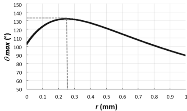
Fig. 22. Expression of \theta_{max} in function of r according to the theoretical model
