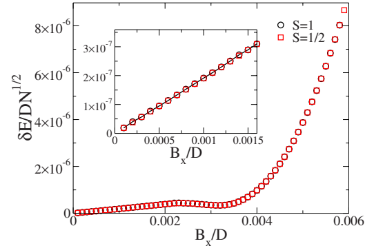
FIG. 2. (Color online) Comparison between the S=1 and S_{\text{eff}} = 1/2 models for a given sample (e.g., realization of disorder) of N=9 spins: gap \delta E / (D\sqrt{N}) as a function of the transverse field B_x/D . \delta E is the energy gap between the two lowest-energy states of the system in presence of both dipolar interactions V_{ij}^{\mu\nu} and the transverse magnetic field B_x . The inset shows the small- B_x/D regime for the same sample.
