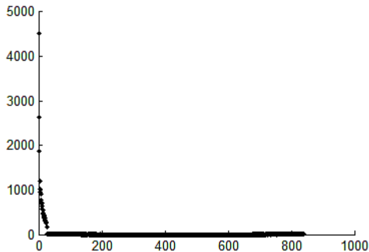
Figure 9. Variances of the 841 PCA-transformed variables in descending order of magnitude
