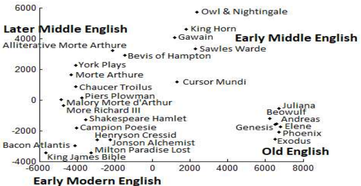
Figure 11: Scatter plot of the two highest-variance variables derived via PCA, with associated text names
