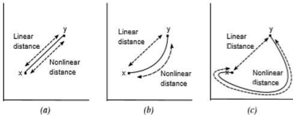
Figure 13. Linear and nonlinear distances on flat and curved manifolds
