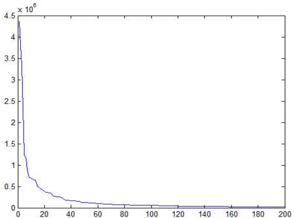
Figure 6. 200 highest-variance columns of M
