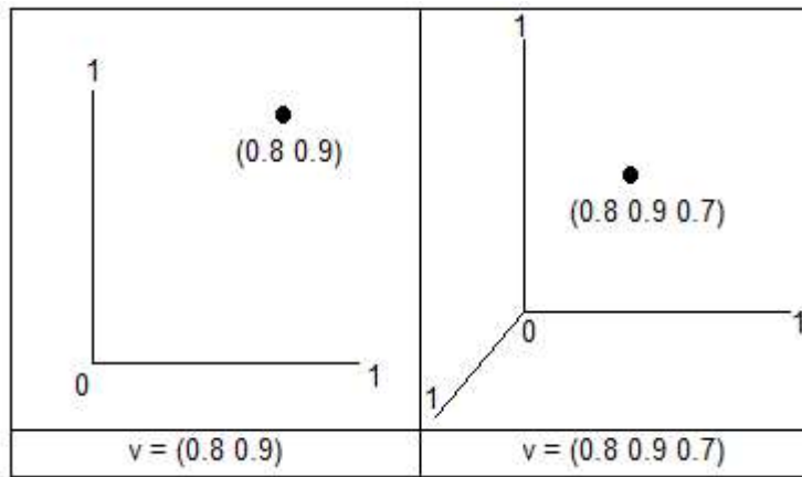
Figure 2. Two and three dimensional vector spaces
