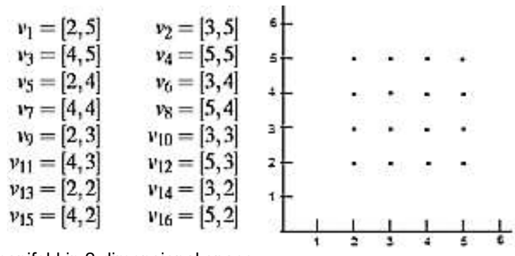
Figure 3. Data manifold in 2-dimensional space
