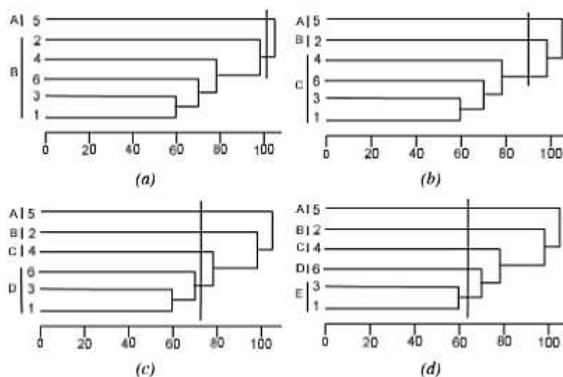
Figure 16. Different 'cuts' of the same tree
