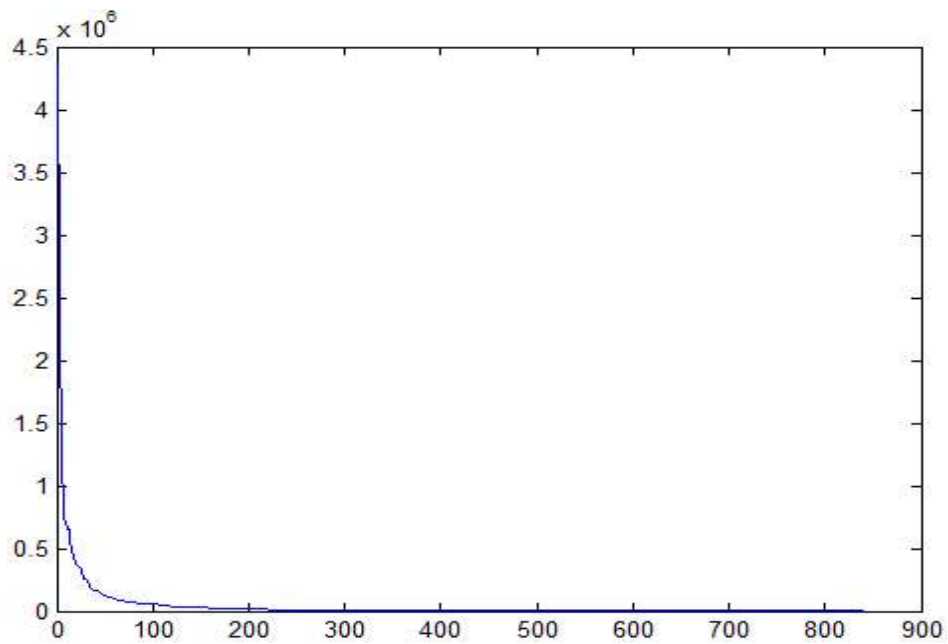
Figure 5. Variances of the columns of M, sorted in descending order of magnitude
