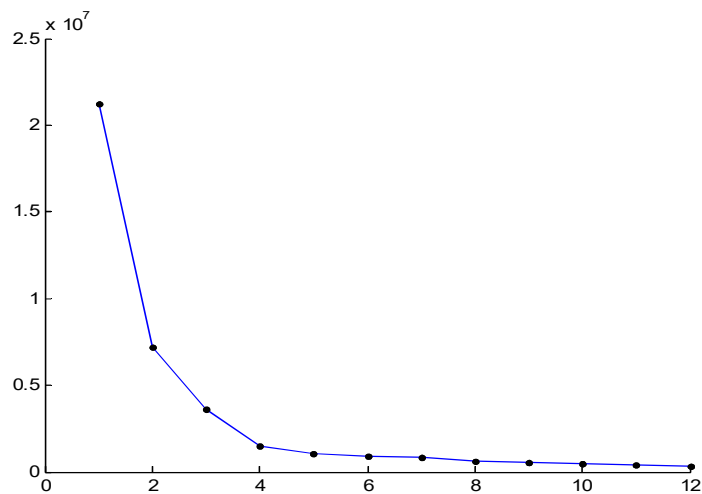
Figure 10. The 12 highest-variance variables in M'
