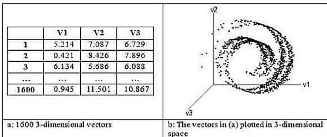
Figure 4. Nonlinear manifold in 3-dimensional space
