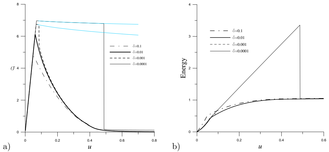
Figure 8: Bar in traction: \Gamma -convergence for different values of \delta obtained without backtracking algorithm. (a) Stress as a function of the imposed displacement; (b) total energy as a function of the displacement.
