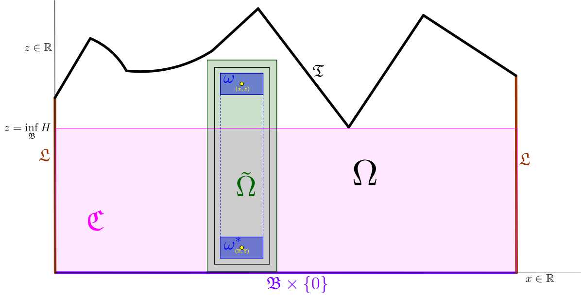
Figure 3: A canonically oriented pseudo-cylinder with a control domain in \Omega \setminus \bar{\mathcal{C}} .
