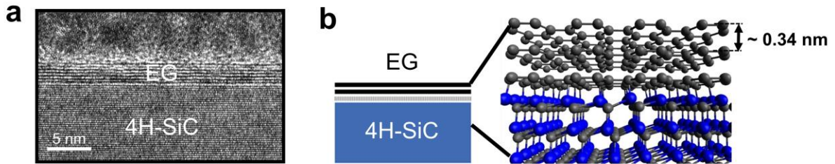
Fig. 1. (a) TEM image and (b) schematic illustration of few-layers epitaxial graphene grown on SiC (0001) substrate by Si sublimation at high temperatures. In the 3D lattice model, it is possible to distinguish the interfacial carbon buffer layer, which is directly bonded to the SiC substrate, and the graphene layers grown on top of it.
