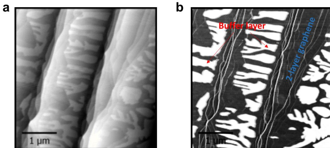
Fig. 3. (a) Contact-mode AFM topographic image (vertical scale: 10 nm) of the 2-L epitaxial graphene sample studied in this work. Higher domains represent the buffer layer. (b) Corresponding friction force image (vertical scale: 50 nN). Thanks to the large difference in their friction response, from the friction map it is possible to clearly distinguish the exposed 2-L epitaxial graphene (low friction-dark contrast) from the buffer layer domains (high friction-brighter contrast). Friction force map has been acquired scanning the sample at 5nN normal load.
