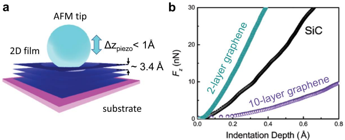
Fig. 2. (a) Schematic illustration of the contact model assumed in the Modulated Nanoindentation (MoNI) technique. The AFM tip can be represented as a sphere indenting locally the 2D film surface, assimilated, together with the substrate, to an elastic half-space. (b) Force versus indentation depths curves obtained from high-resolution Modulated Nanoindentation (MoNI) measurements, showing the mechanical responses of epitaxial graphene films of different thicknesses, compared to that of the SiC substrate.
