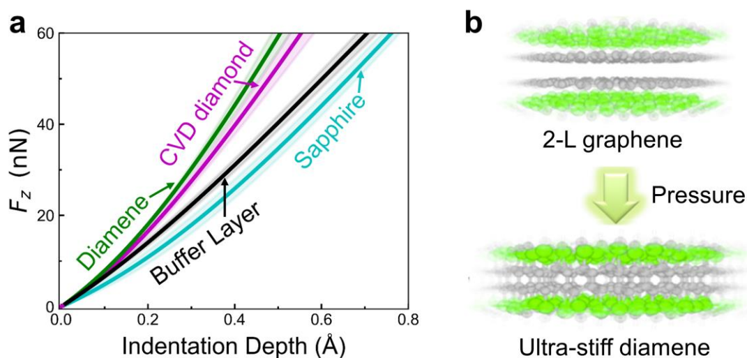
Fig. 4. (a) Force versus indentation depth curves obtained from MoNI experiments on 2-L epitaxial graphene on SiC(0001) and on different hard materials. The curves plotted are the result of an averaging process of data extracted from different positions on the surface of each sample. Shaded areas represent the respective standard deviations from the mean value. All the measurements are performed using the same diamond tip. The reported experiment clearly shows that the diamene/SiC structure (green line) exhibits a stiffness larger than that of CVD bulk diamond (magenta line). (b) Illustration of a 2-L epitaxial graphene film on SiC (represented by the bottom green atomic plane), undergoing the phase transition to a diamond-like structure (diamene) under the effect of compression exerted by the AFM tip (upper green atomic plane).
