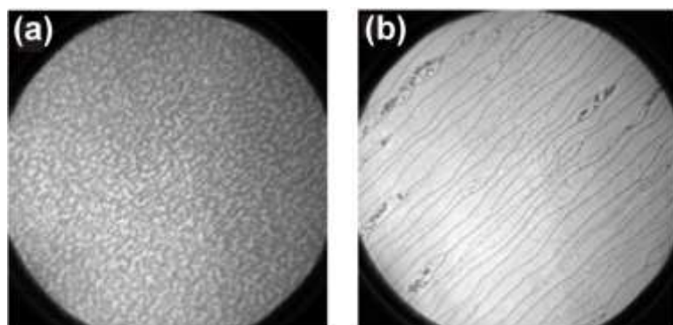
Fig. IV.4. Epitaxial graphene layers grown on the Si-face (a) in vacuum, (b) under Ar [542]; the lines are identified as bilayer graphene [543]. Adapted from [542] and [543].
