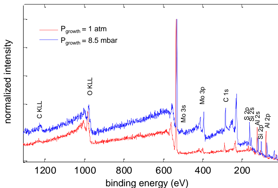
Figure VII.14. XPS survey spectra of \text{MoS}_2/\text{sapphire} samples from the two growth runs with different chamber pressures (1 atm and 8.5 mbar). XPS measurements were performed with PHI Versaprobe II equipped with X-ray source, \text{Al K}\alpha ; h\nu = 1486.6 \text{ eV} .
