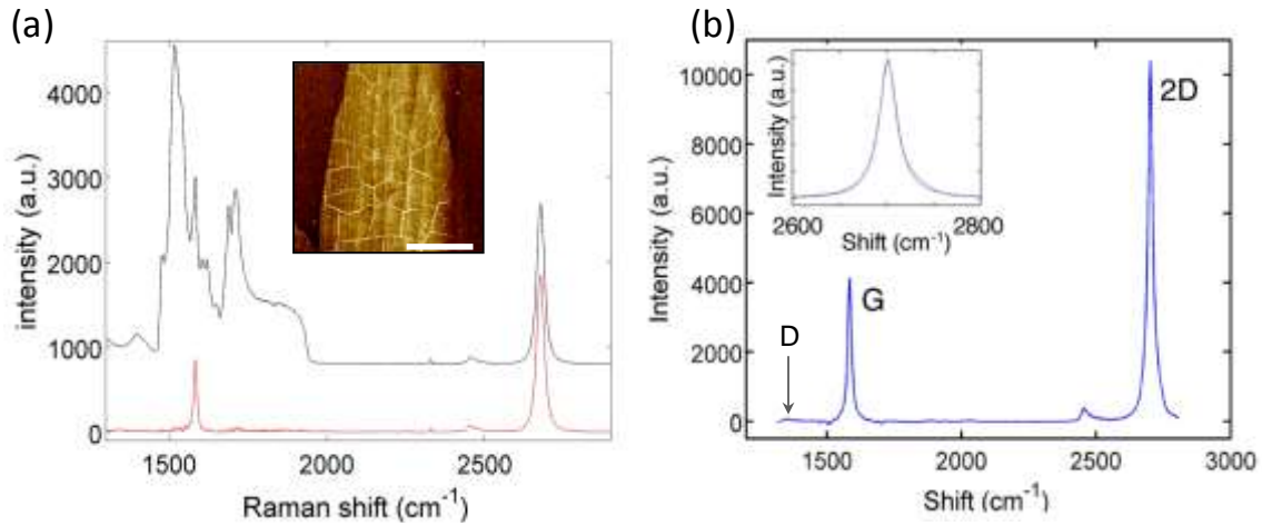
Fig. IV.7. Raman spectroscopy for graphene layers on 4H-SiC C-face (a) monolayer graphene, (b) multilayer graphene, with the Raman contribution for SiC removed. Note the absence of the D peak. In (a) the black trace is the raw data, the red trace is the graphene spectrum once the SiC Raman peaks have been subtracted by the Non-negative Matrix Factorization method [584]. In (b) the inset shows a Lorentzian 2D peak for this ten layer sample. Figure adapted from Ref [583].
