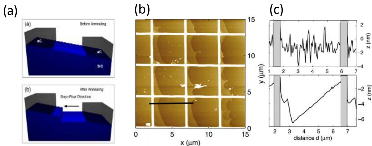
Fig. IV.9. SiC Step pinning under an evaporated amorphous carbon grid. (a) Schematics of step pinning. After annealing at 1350°C, the steps accumulate at one side of the grid in each enclosure providing large terraces at a locations defined by the grid. (b) AFM image and (c) topographic profile within the grid (top) before and (bottom) after step bunching annealing, showing that a large terrace has developed. Adapted from [595].
