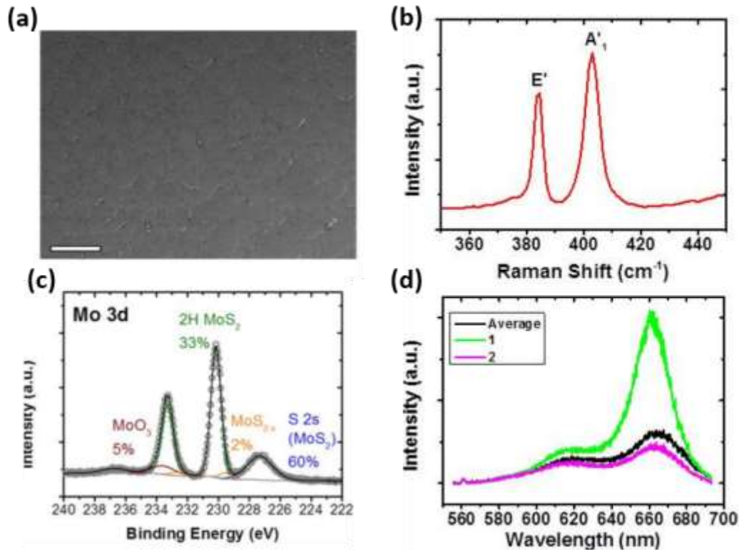
Fig. VII.7: (a) SEM image showing continuous MoS 2 film. Scale bar is 2 μm. (b) Average Raman spectrum measured across a 20x20 μm area of the film. (c) Mo 3d core level showing contributions consistent with MoS 2 . (d) PL measured across monolayer region (green) and bilayer island (pink). Adapted from Ref [903].
