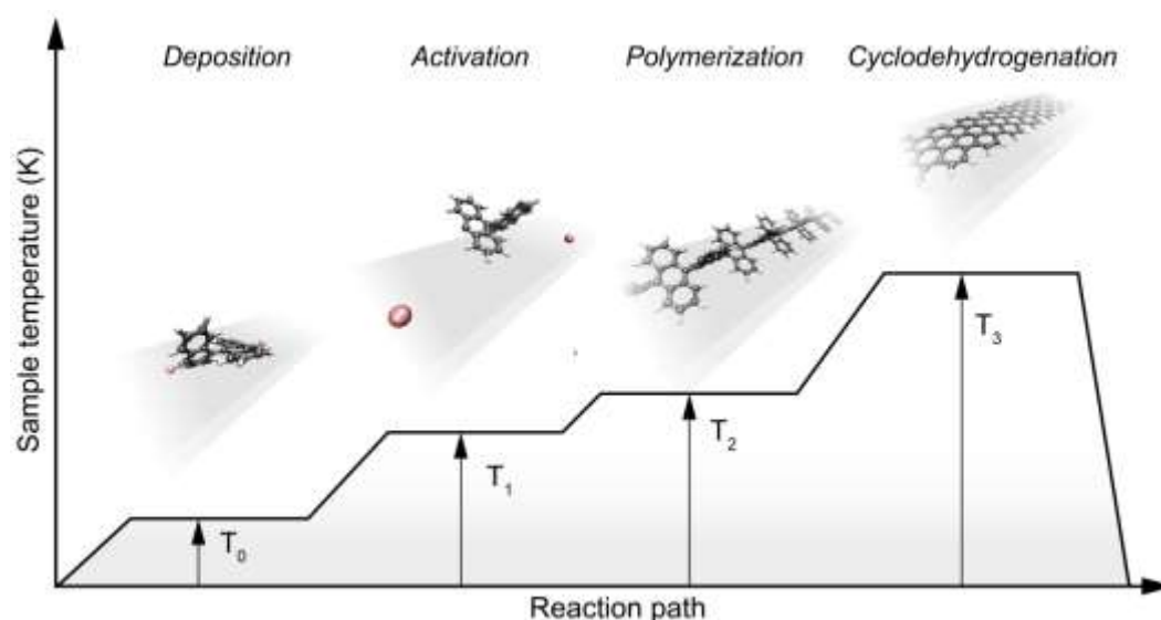
Fig. I.1: GNR bottom-up synthesis concept. GNR synthesis is achieved by deposition of halogen-substituted precursor monomers at a substrate temperature T_0 , followed by their activation (halogen cleavage) at T_1 , polymerization at T_2 , and cyclodehydrogenation at T_3 .
