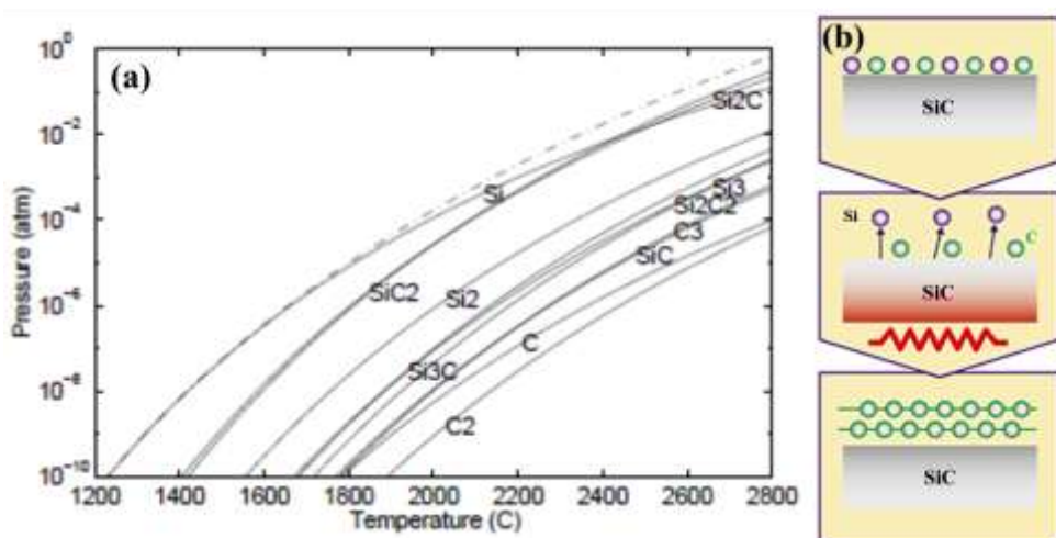
Fig. IV.2. (a) Partial pressure of different vapour species vs. temperature in equilibrium with a crystal on SiC. (b) Schematics of graphene formation by Si sublimation[560].
