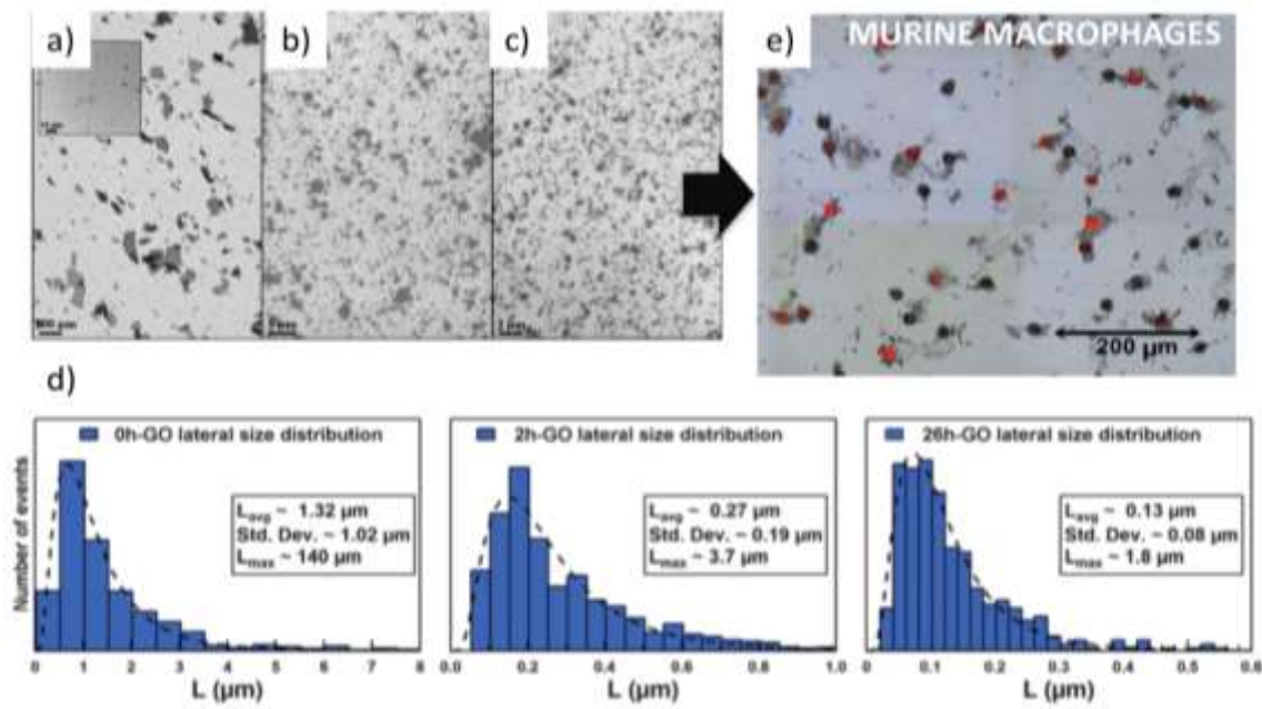
Fig. II.13: a,b,c) SEM image of GO solutions sonicated for different times, then spin coated on 300 nm SiO_2/Si(100) : 0 h-GO (a), 2 h-GO (b), and 26 h-GO (c). d) Flake size distribution of the 0 h-GO, 2 h-GO and 26 h-GO samples from SEM statistics. e) Optical map of mIPM cells incubated with GO. Red dots indicate where Raman spectra was taken to detect internalization of GO into the cell. Adapted from Ref. [279].
