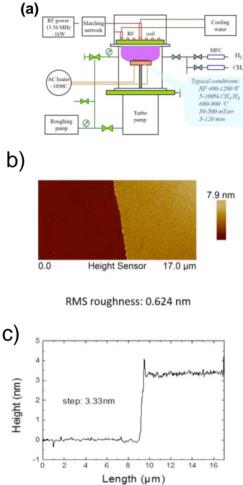
Fig V.34. (a) Schematic PECVD system used to grow graphene films on Si/SiO 2 . Figure reproduced from Ref. [833] (b) AFM image of the grown graphene film (c) Height profile.
