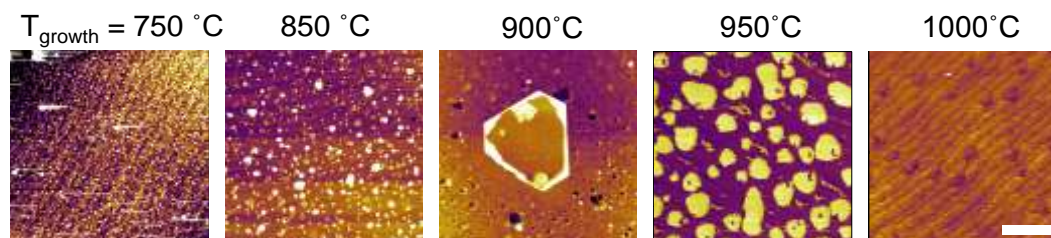
Fig. VII.11. Temperature-dependent growth morphology illustrated by AFM height images of as-grown \text{MoS}_2 sapphire samples produced at different growth temperatures. Scale bar, 250 nm. Adapted from ref. [921].
