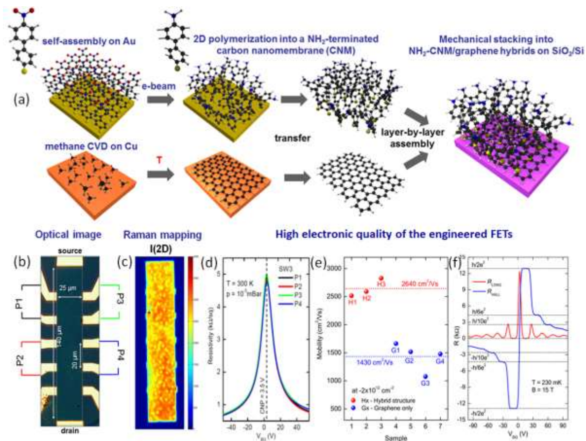
Fig. VIII. 10: Non-destructive chemical functionalization of SLG. a) Schematic of the fabrication of NH 2 -CNM/SLG heterostructures via mechanical stacking of the individual sheets. b) Microscope image of the fabricated FET with Au contacts in the Hall bar geometry. c) Mapping of the Raman 2D peak on the active device area. d) RT homogeneous electrical field effect at different side contacts of the FET as a function of V_G . e) Mobility of heterostructure and reference devices. f) Quantum oscillations in a magnetic field at low T confirming high electronic quality of SLG in the fabricated heterostructures. Adapted from ref [1100]
