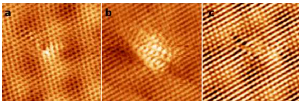
Fig. IX.25: Three 5 \times 5 \text{ nm}^2 images showing 0-D graphene point defects on Pt(111). a. 10 \text{ mV} , 3.9 \text{ nA} . b. 10 \text{ mV} , 2 \text{ nA} . c. 10 \text{ mV} , 3.9 \text{ nA} . See main text for detailed description.
