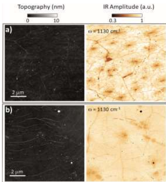
Fig. VI.8 AFM and near-field IR images recorded from samples before (a) and after (b) heat treatment. Scan size for each measurement was 10 \times 10 \mu\text{m}^2 . Courtesy of Dr. Adrian Cernescu, Neaspeck GmbH Germany.
