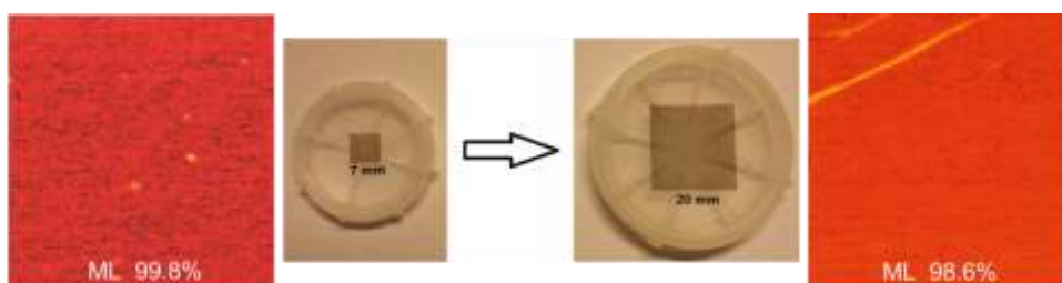
Fig. IV.12. Size increase of monolayer graphene samples from 7 \times 7 \text{ mm}^2 to 20 \times 20 \text{ mm}^2 . The size of reflectance maps (red scale) are 30 \mu\text{m} \times 30 \mu\text{m} [596].
