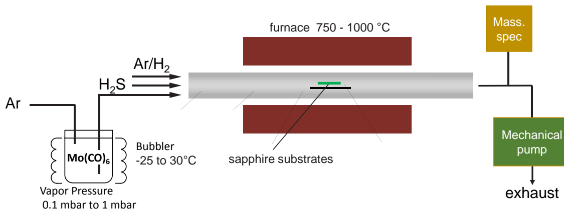
Fig. VII.10. The schematic of our MOCVD setup. Note the reverse bubbler configuration in the Mo(CO) 6 .
