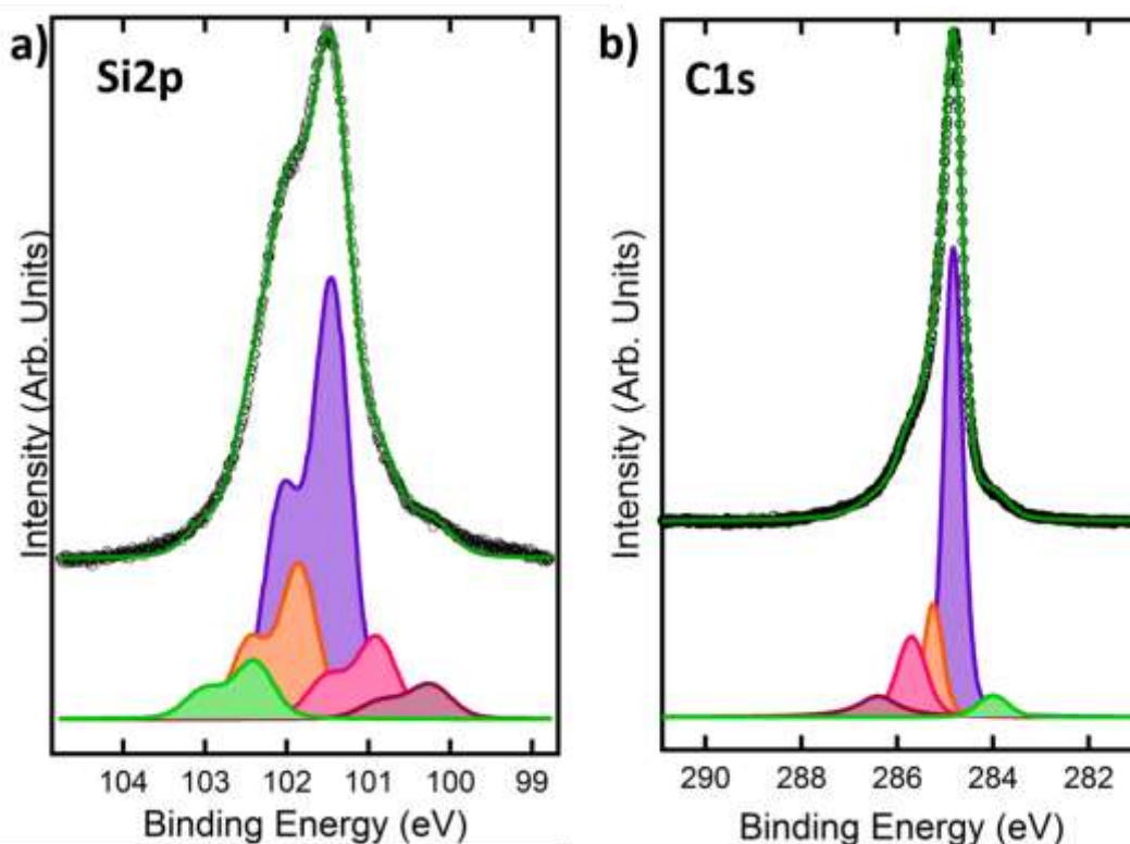
Fig. IX.50: a) XPS Spectrum of Si2p peak of SLG/SiC annealed at 1400K recorded with a photon energy of 150 eV. b) XPS spectrum of C1s peak of SLG/SiC annealed at 1400K recorded at 400 eV.
