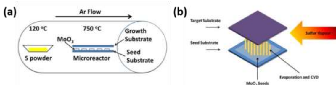
Fig. VII.6: (a) Schematic of the set-up for CVD of \text{MoS}_2 . (b) Illustration of the mechanism by which \text{MoS}_2 is deposited on the target substrate. Adapted from Ref [903].
