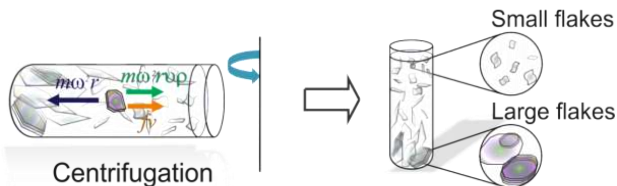
Fig. III.1: Sorting of GRM flakes by ultracentrifugation. The SBS approach allows separating thin and small lateral sized flakes (supernatant) from thicker and larger ones, which precipitate at the bottom of the ultracentrifuge tube as pellet. The actual nanosheet dimensions (lateral size, layer number) depend on the centrifugal acceleration, material and medium.
