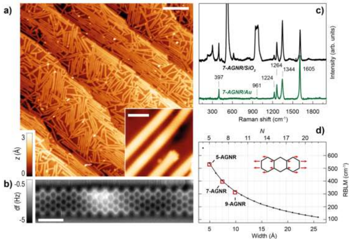
Fig. I. 3: Characterization of 7-AGNRs on their growth substrate and after substrate transfer. a) Large-scale STM topography image (Bias: -0.5 V; Current: 5 pA; T: 4.5 K; Scale bar: 30 nm) showing high coverage 7-AGNRs on Au(111). Inset: small-scale STM image (Bias: 0.1 V; Current: 30 pA; Scale bar: 3 nm). The apparent height of individual 7-AGNRs is 0.19 nm. (b) Constant-height nc-AFM frequency shift image (Bias: 2 mV; Oscillation amplitude: 0.3 Å; T: 4.5 K; Scale bar: 1 nm) taken with a CO-functionalized tip. (c) Raman spectra of 7-AGNR on Au(111) recorded under ambient conditions immediately after synthesis (green curve) with indicated peak positions of the main lines, and after transfer to Si/SiO 2 (black curve; laser 532nm, power of 2mW, 3 scans of 20 seconds). (d) RBLM peak position for 5-AGNRs, 7-AGNRs and 9-AGNRs (red markers), together with predicted width-dependent RBLM wavenumbers for AGNRs [45].
