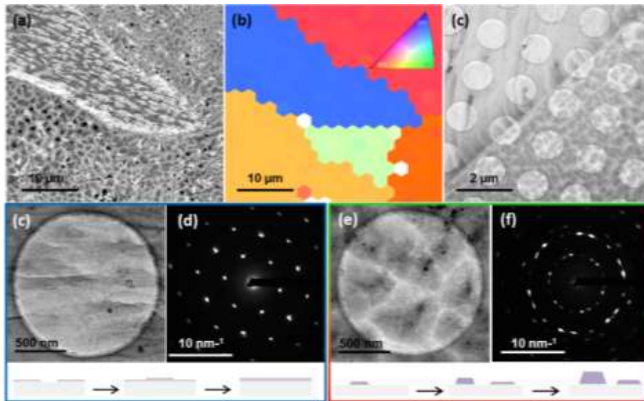
Fig. VII.5: (a) SEM image and (b) the corresponding EBSD mapping of the BN film on nickel substrate. (c) TEM image of the BN film transferred by the polymer-free technique on holey amorphous carbon film TEM grid. High-resolved TEM images and the corresponding electron diffractions of (d) and (e) a flat BN area and (f) a rough BN area with the schematic of the growth process: Van der Merwe for Ni(111) and Volmer Weber for Ni(110) and Ni(001).
