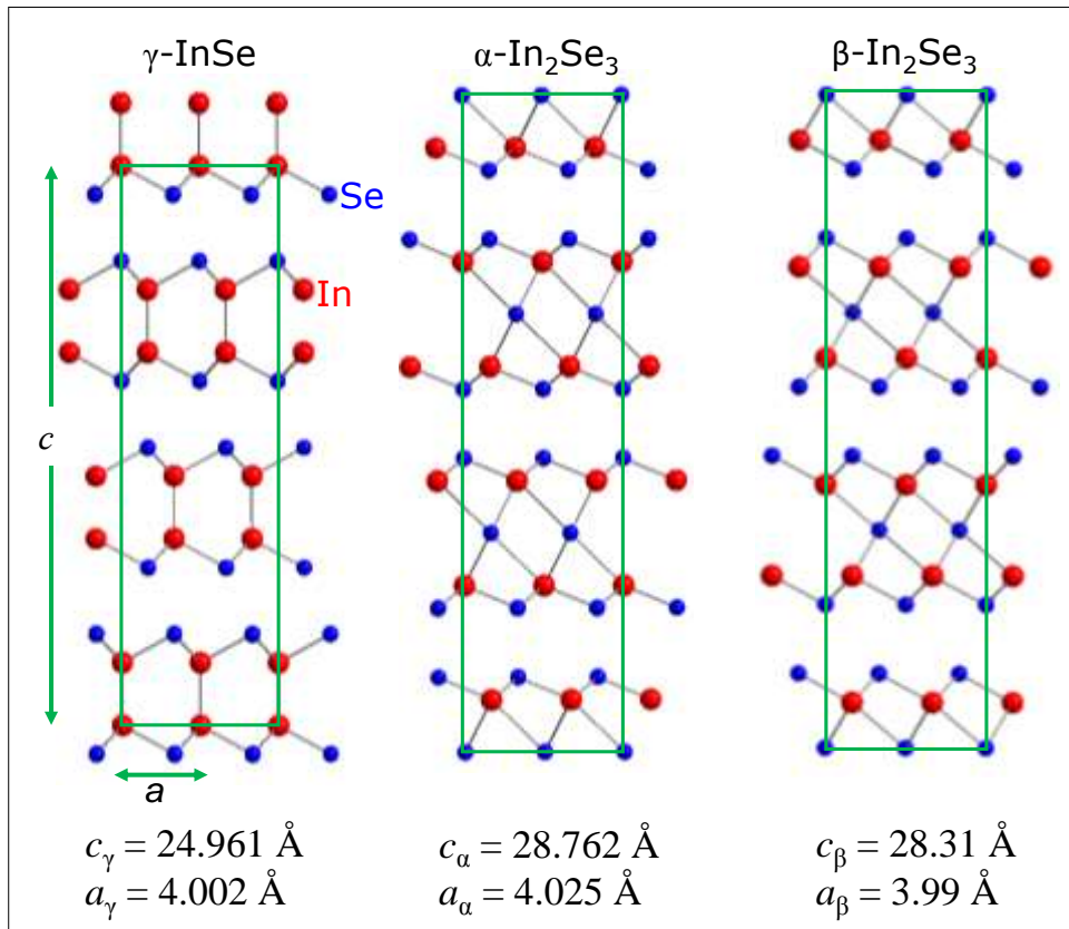
Fig VII.20: Side view of the crystal lattice and unit cell of \gamma -InSe (left), \alpha - \text{In}_2\text{Se}_3 (middle) and \beta - \text{In}_2\text{Se}_3 (right). Blue and red spheres correspond to Se- and In-atoms, respectively. The primitive unit cell of \gamma -InSe contains three layers, each consisting of four closely-packed, covalently bonded, atomic sheets in the sequence Se-In-In-Se. For both \alpha - and \beta - \text{In}_2\text{Se}_3 phases, the primitive unit cell contains three layers, each consisting of five closely-packed, covalently bonded, atomic sheets in the sequence Se-In-Se-In-Se. In \alpha - \text{In}_2\text{Se}_3 the outer Se-atoms in each layer are aligned, whereas in \beta - \text{In}_2\text{Se}_3 they are located into the interstitial sites of the Se-atoms in the neighboring layers, thus leading to a smaller volume in \beta - \text{In}_2\text{Se}_3 .
