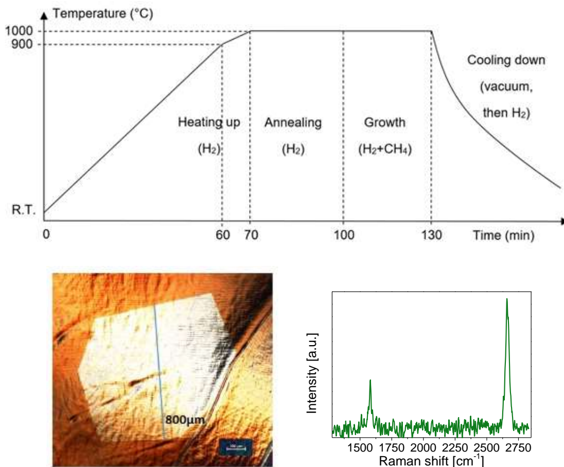
Fig. V.2 Upper – typical schematics of thermal profile during the growth, type of gases used and steps duration in case of growth SLG at 1000\ ^\circ C , (Lower Left) Optical image of a graphene domain grown on molten Cu ( 1020\ ^\circ C ) on a molybdenum substrate. Scale bar is 100\ \mu m . (Lower Right) Raman spectrum of a graphene domain grown on molten Cu.
