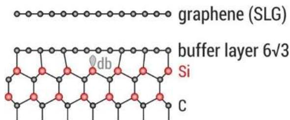
Fig .IV.21. Schematic view of epigraphene on SiC(0001), also referred to as SLG. The graphene layer resides on top of the buffer layer. The buffer layer is structurally equivalent to graphene but strongly bound to the SiC substrate. Dangling bonds (db) may be present due to the lattice mismatch between graphene and SiC. Drawing not to scale (After [598, 625]).
