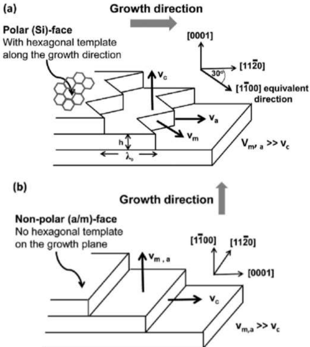
Fig. IV.20. Graphene growth mechanism on (a) the polar (Si) face SiC with offcut toward [11\bar{2}0] and (b) the nonpolar a/m face with slight offcut along [0001] . The EG growth on the polar face proceeds laterally while the EG growth on the nonpolar face is limited by the vertical growth rate. The zigzag structure shown on the polar face step edge is a consequence of two possible lateral growth directions. (Adapted from Ref. [622])
