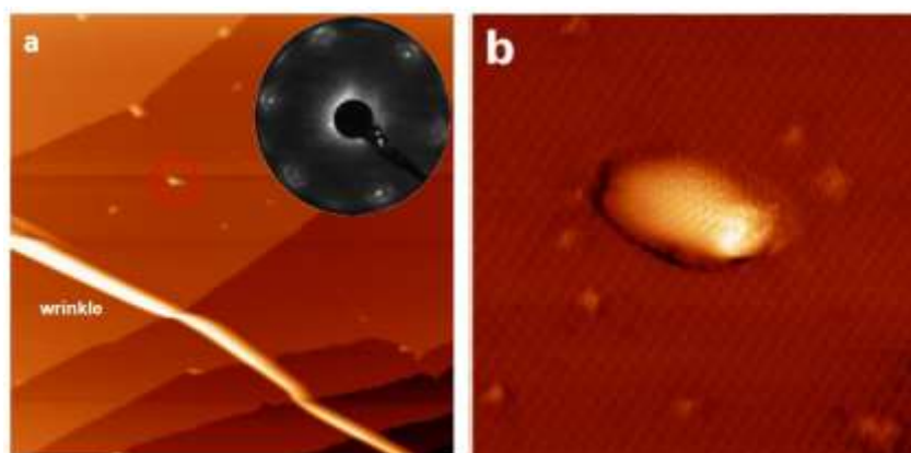
Fig. IX.24 .a) STM image of a 200 \times 200 \text{ nm}^2 area of graphene epitaxially grown on Pt(111), I=0.15 \text{ nA} , V=750 \text{ mV} . A single graphene layer covers the whole surface. In the image a wrinkle/pleat and several nanobubbles one of them is encircled in red, can be seen. The inset shows the characteristic LEED pattern of Gr on Pt(111). b) High resolution STM image of a graphene nanobubble ( 20 \times 20 \text{ nm}^2 , I=0.6 \text{ nA} , V=310 \text{ mV} ) and few point-like atomic defects with atomic resolution. Figure a is adapted from reference [875].
