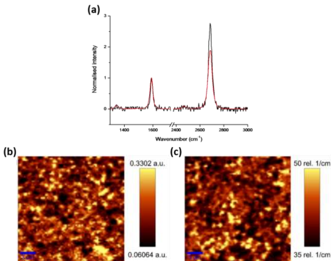
Fig. V.16 (a) Raman spectrum taken at the centre of a monolayer graphene domain (black) and averaged across a 20 \times 20 \mu\text{m} region of the film (red). (b) I_D/I_G map. (c) 2D FWHM map. Adapted from [755]
