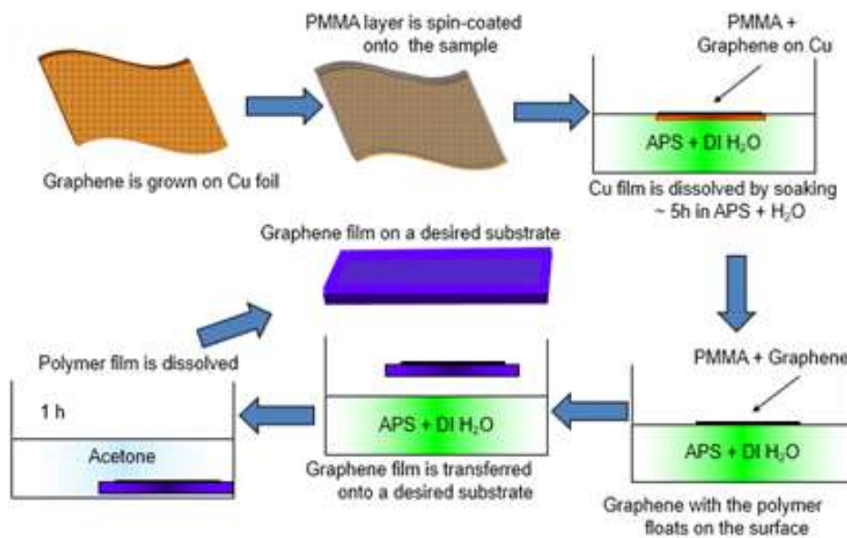
Fig. VI.1 Wet transfer procedure
