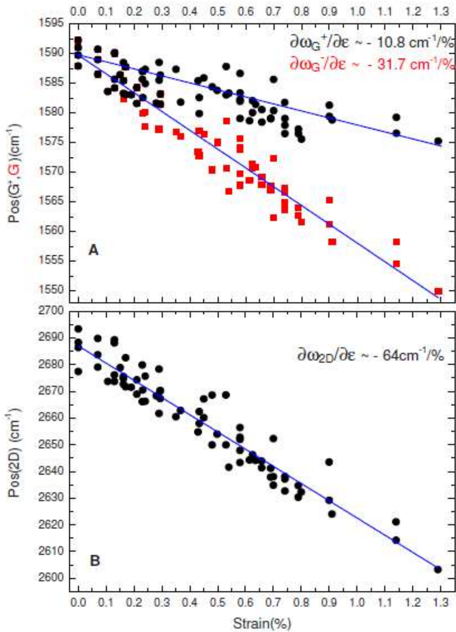
Fig IX.40: Change in \text{Pos}(G) and \text{Pos}(2D) with increasing amount of tensile, uniaxial strain. Fig. adapted from [1306].
