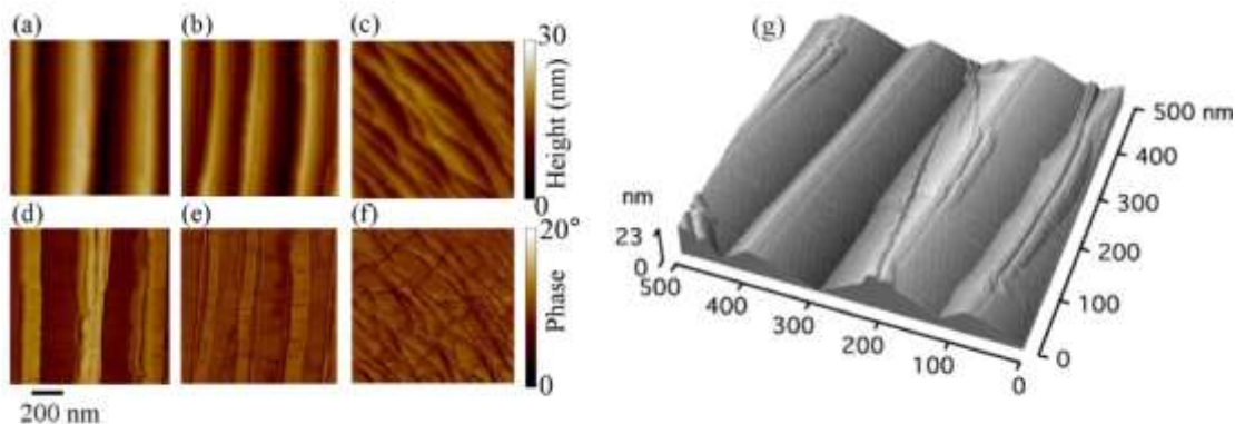
Fig. IV.15. (left panel) AFM images. Effect of graphitization temperature on the surface morphology of the sample 8^\circ -off axis (0001) 4H-SiC: 1600°C (a), 1700°C (b) and 2000°C (c). The phase contrast maps
