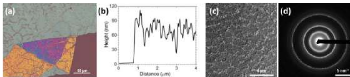
Fig. VII.4: (a) optical image of BN film grown on copper and transfer onto 90 nm \text{SiO}_2/\text{Si} , scale bar is 50 \mu\text{m} . (b) AFM profile showing the 90 nm thickness and the high roughness of the BN film. (c) TEM image with scale bar 4 \mu\text{m} and (d) electron diffraction pattern showing the rough/turbostratic behavior of the multilayers BN film grown on copper with scale bar 5 \text{nm}^{-1} .
