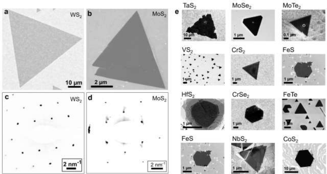
Fig. VII.26. SEM images of (a) WS_2 and (b) MoS_2 . TEM diffraction patterns of WS_2 (c) and MoS_2 (d) crystals after transfer onto TEM chips indicate monocrystallinity. (e) Selection of 12 binary compounds grown with the same method and similar process conditions.
