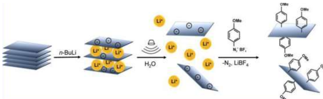
Fig. VIII.17: Schematic of the basal-plane functionalization of MoS 2 . After intercalation with n -butyllithium, the negatively charged MoS 2 is dispersed in water by mild bath-type sonication leading to an efficient exfoliation into individual sheets. The charges on the MoS 2 are quenched by the addition of 4-methoxyphenyldiazonium tetrafluoroborate obtaining the functionalized product. Adapted from Ref [350]
