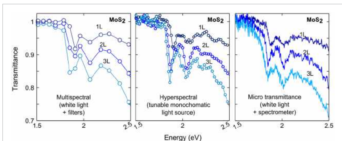
Figure IX.10. Comparison between different methods to measure the optical properties of 1L,2L,3L-MoS 2 . In multispectral imaging narrow bandwidth filters (10 nm FWHM) are used to select the wavelength (the wavelength resolution is limited by the number of filters). In hyperspectral imaging, the illumination is provided through a white light source connected to a monochromator (2–3 nm resolution). In micro-transmittance, white light is collected through an optical fiber (acting as a confocal pinhole) and sent to a CCD spectrometer (~1 nm resolution). Adapted from [1436].
