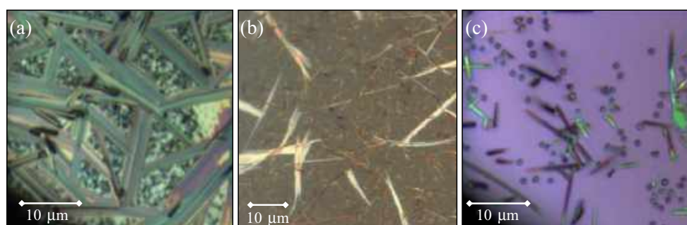
Figure VII.14. Optical micrographs of \beta - \text{In}_2\text{Se}_3 rods (a) grown on mica at T = 620^\circ\text{C} for t = 9\text{ h} under an Ar flow rate of 150 sccm, (b) grown on mica at T = 570^\circ\text{C} for t = 6\text{ h} under an Ar flow rate of 150 sccm, and (c) grown on \text{Si}/\text{SiO}_2 at T = 600^\circ\text{C} for t = 6\text{ h} under an Ar flow rate of 170 sccm.
