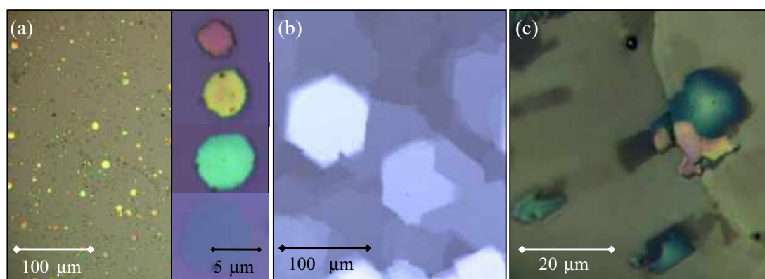
Figure VII.13. Optical micrographs of \beta - \text{In}_2\text{Se}_3 layers grown on (a) \text{SiO}_2/\text{Si} , (b) mica, and (c) graphite ( T = 600^\circ\text{C} , t = 9\text{ h} and Ar flow rate \sim 150\text{ sccm} ). Different colors correspond to different thicknesses of the layers. This ranges from hundreds of nanometers down to 2.8 nm. Adapted from [1117], © IOP Publishing Ltd.
