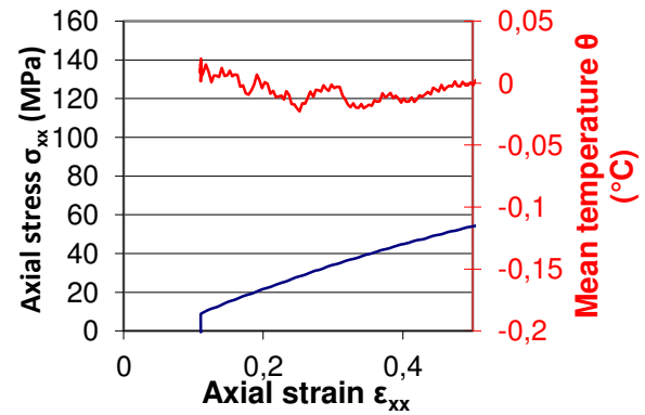
Figure 5. Zoom on results of tensile tests on [\pm 45]_s carbon/epoxy laminate between \varepsilon_{xx} = 0 and \varepsilon_{xx} = 0,5
