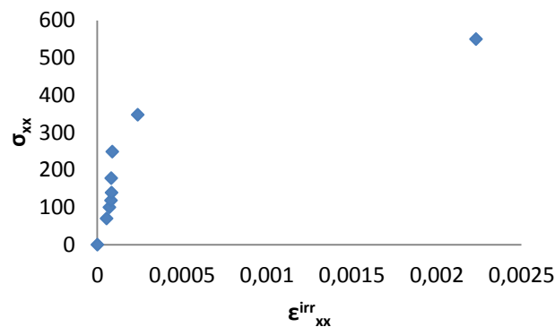
Figure 9. Stress versus irreversible strain curve for quasi-isotropic carbon/epoxy laminate (stratification [\pm 45/90/0]_s )
