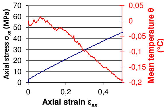
Figure 4. Zoom on results of tensile tests on [\pm 67,5]_s carbon/epoxy laminate between \varepsilon_{xx} = 0 and \varepsilon_{xx} = 0,5
