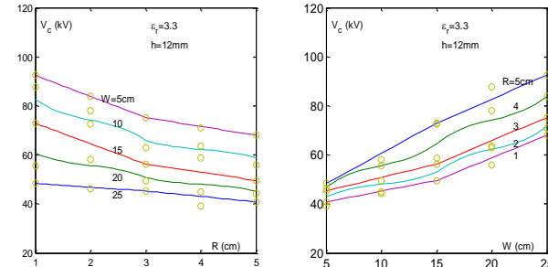
Fig. 11. Influence of the position and the width of the barrier on the DC voltage disruptive voltage for the hole H=12\text{ mm} and the relative permittivity \epsilon_r = 3.3
