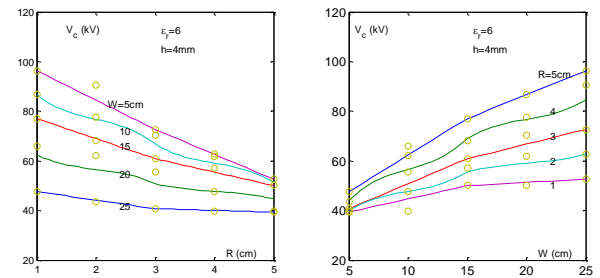
Fig. 10. Influence of the position and the width of the barrier on the DC voltage disruptive voltage for the hole H=4\text{ mm} and the relative permittivity \epsilon_r = 6
