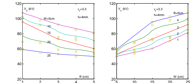
Fig. 12. Influence of the position and the width of the barrier on the DC voltage disruptive voltage for the hole H=4\text{ mm} and the relative permittivity \epsilon_r = 3.3
