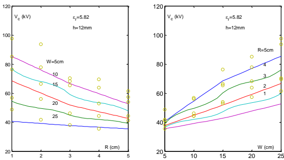
Fig. 14. Prediction of the breakdown voltage in terms of R and W for the hole H=12\text{ mm} and the relative permittivity \epsilon_r = 5.82
