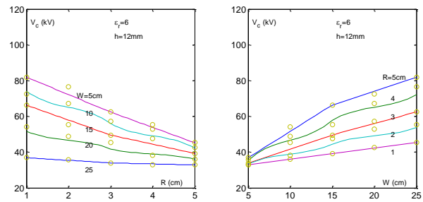
Fig. 9. Influence of the position and the width of the barrier on the DC voltage disruptive voltage for the hole H=12\text{ mm} and the relative permittivity \epsilon_r = 6
