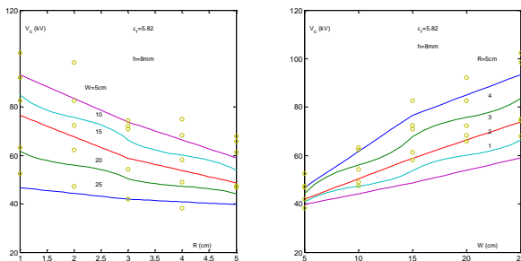
Fig. 15. Prediction of the breakdown voltage in terms of R and W for the hole H=8\text{ mm} and the relative permittivity \epsilon_r = 5.82
