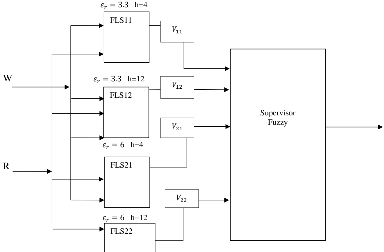
Fig. 8. Supervisor fuzzy
