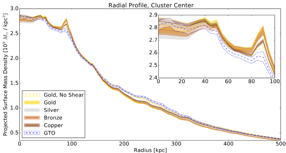
Figure 9. Radial surface mass density profiles of all models. In each case the best-fitting value is shown by a dark line, surrounded by a lighter shaded region representing model uncertainty. The shape of the profile is similar for all models: The surface density is largely flat in the central cluster core and then slowly diminishes at larger radii. This is also consistent with other independent models of A370 (e.g. D18), and we do expect a flat core, based on the high number of multiple images seen near the cluster centre (Section 3.3.1). The sharp peak at \sim 90 kpc is due to the high mass of the BCGs, which are considerably overdense compared to other components. The total magnitude of the density is also largely consistent between models in the inner cluster, given the measured errors, though the GTO and ‘no-shear’ gold models show higher densities at distances beyond 200 kpc. This is because these models do not utilize a (massless) external shear term, and the discrepancy between the sheared and non-sheared models can point to the presence of additional mass components in the cluster outskirts. In the inset plot we zoom in on the central 100 kpc of the cluster, better differentiating the profile shape of different models and highlighting their good statistical agreement.
