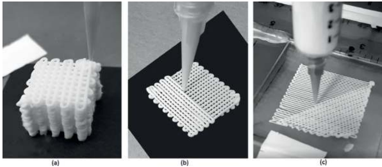
Figure 2. 3D printed scaffolds using three types of nozzles: (a) \text{\O} 0.8 mm; (b) \text{\O} 0.6 mm; and (c) \text{\O} 0.4 mm [95].
