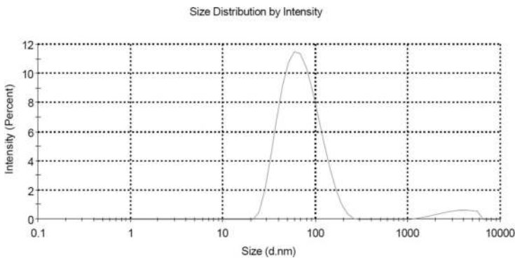
Figure 6. Particle size distribution of one hybrid sample filtered through 0.22 μm Millipore membrane.
