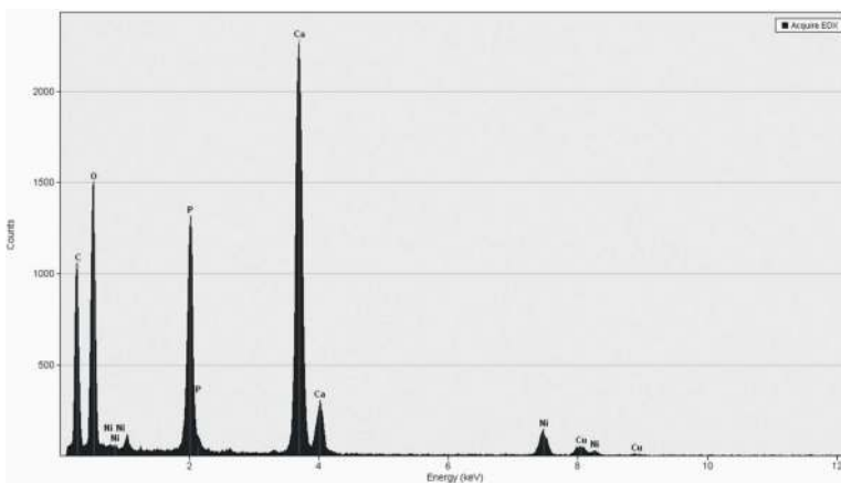
Figure 8. EDX spectra of one hybrid sample with 80% HA and 20% PU.
