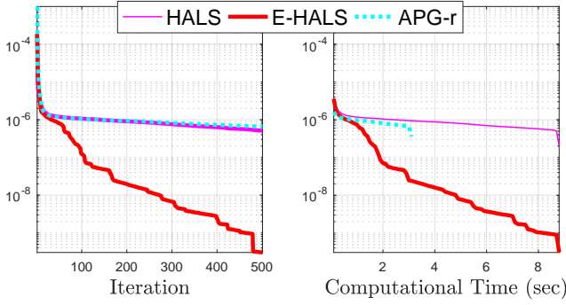
FIGURE 2 – Median value of e^k - e_{\min} of HALS, E-HALS and APG-r for test 2.
