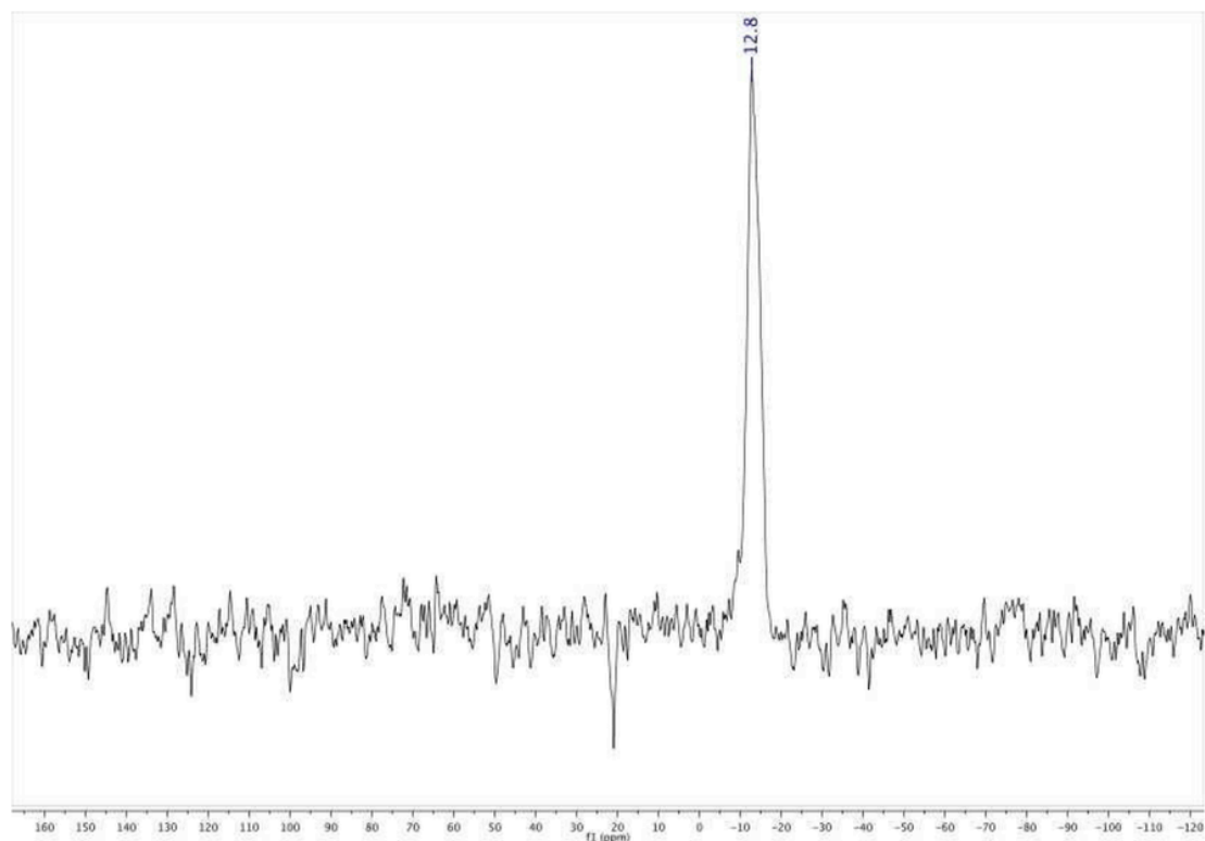
Fig. 8. ^{31}\text{P} CP-MAS NMR spectrum of 2 @ \{\text{NH}_2\} -SBA-15.
