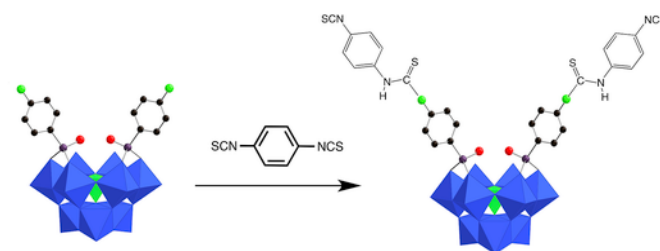
Fig. 2. Synthetic route for post-functionalization of (^n\text{Bu}_4\text{N})_3[\text{NaHPW}_9\text{O}_{34}\{\text{As}(\text{O})\text{C}_6\text{H}_4-\text{NH}_2\}_2] (1) by PDITC leading to the formation of compound 2.
