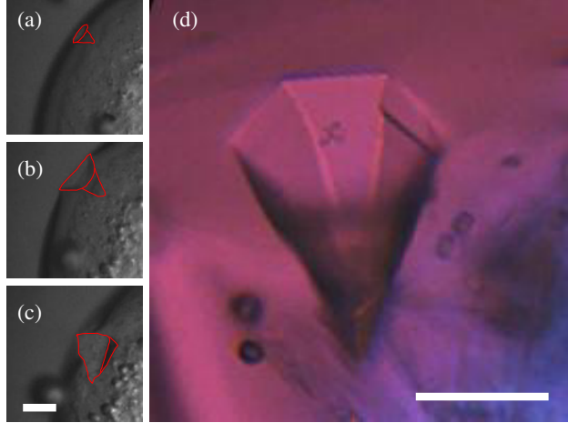
Figure 7: (a-c) Growth of a conical hydrate crystal in a solution of CP with 0.1% Span 80 over 22 seconds during the temperature plateau at T = 0.2^\circ\text{C} (273.35 K). The red outlines identifies typical hydrate crystals borders and the scale bar represents 100\ \mu\text{m} . (d) View of the conical crystal through polarized light microscopy. The scale bar represents 25\ \mu\text{m} .
