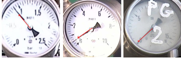
Fig. 8: Examples of correct needle detection in manometers in non-optimal conditions.
