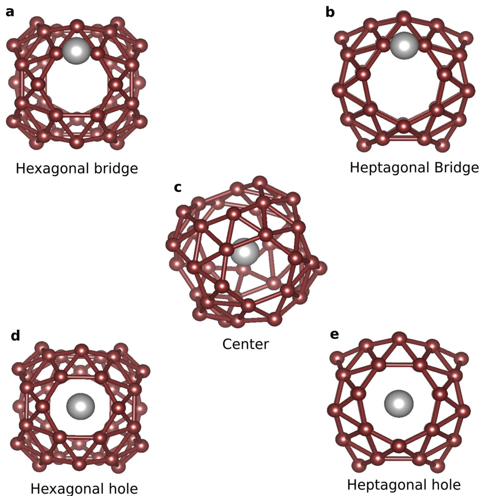
Figure 1. The adsorbate atom, represented by grey ball, can be placed on five different positions in the borospherene ( B_{40} ) represented by brown balls. The five different sites are (a) on the B-B bond of the hexagonal ring, (b) on the B-B bond of the heptagonal ring, (c) center of the cage, (d) hexagonal hole and (e) heptagonal hole.
