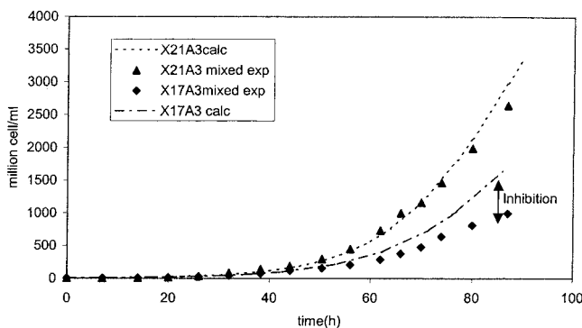
Figure 5. Comparison of the biomass concentrations of strains in pure and mixed cultures 21A3–17A3.
