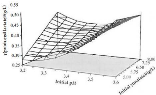
Fig. 3. Produced lactate versus initial values of pH and malate concentrations
