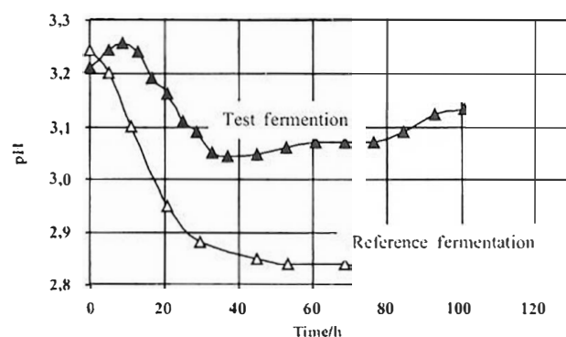
Fig. 7. pH evolution for the reference fermentation and the fermentation carried out with 5 g/L of malic acid
