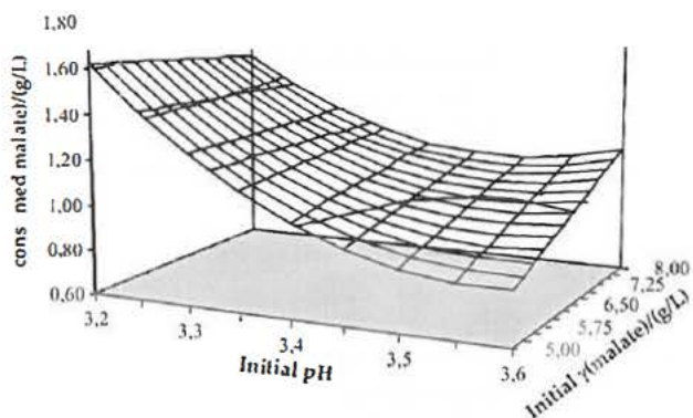
Fig. 1. Consumed malate versus initial values of pH and malate concentrations
