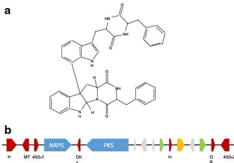
Fig. 4 Asperazine biosynthesis in A. tubingensis G131 a. Asperazine structure b. Schematic representation of the putative asperazine SM cluster (cluster 46). Arrows indicate putative genes in the cluster and its direction indicates forward and reverse strand. Blue: gene coding for a backbone enzyme, Red: gene coding for an enzyme with known function, Green: gene coding for a transcription factor, Yellow: gene coding for a transporter, Grey: gene coding for an hypothetical protein. Below each biosynthetic gene, the putative function is indicated. Dh: dehydratase, H: hydrolase, OR: oxidoreductase, MT: methyltransferase, 450: cytochrome P450
