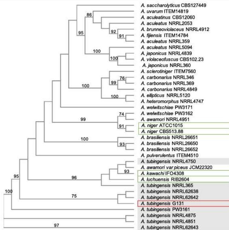
Fig. 2 Phylogenetic tree produced from the combined sequence data of three loci ( pbp2 , benA , cam1 ) of 38 strains of uniseriate black Aspergilli. Numbers above branches are bootstrap values. Only those above 70% are indicated. The evolutionary history was inferred using the Neighbour Joining method computed with the Maximum Likelihood Evolutionary method. Grey background highlighted A. tubingensis strains; Green frame highlighted the genome used for the comparative analysis of this study; Red frame highlighted the genome sequenced in this study
