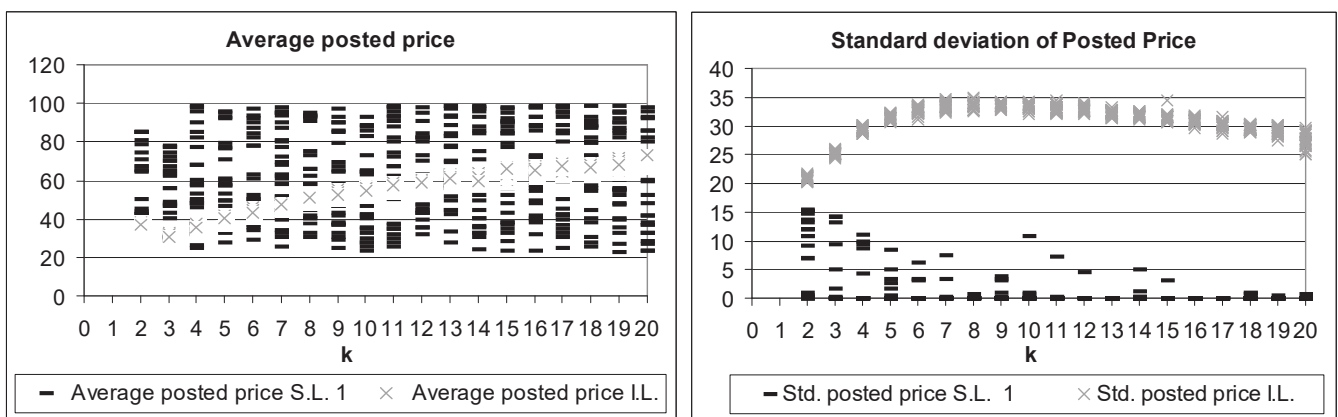
Figure 10. Average price and price dispersion; comparison between IL and SL for different values of k , a=0.9 . (25 simulations for each parameter k and learning type)
