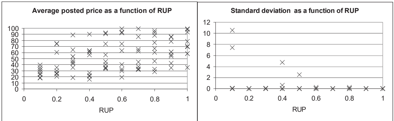
Fig. 14. Average price and standard deviation for \tau = 0.05 and \alpha ranging from 0 to 1. (9 simulations for each parameter configuration (temperature \tau , reward updating parameter \alpha ))
